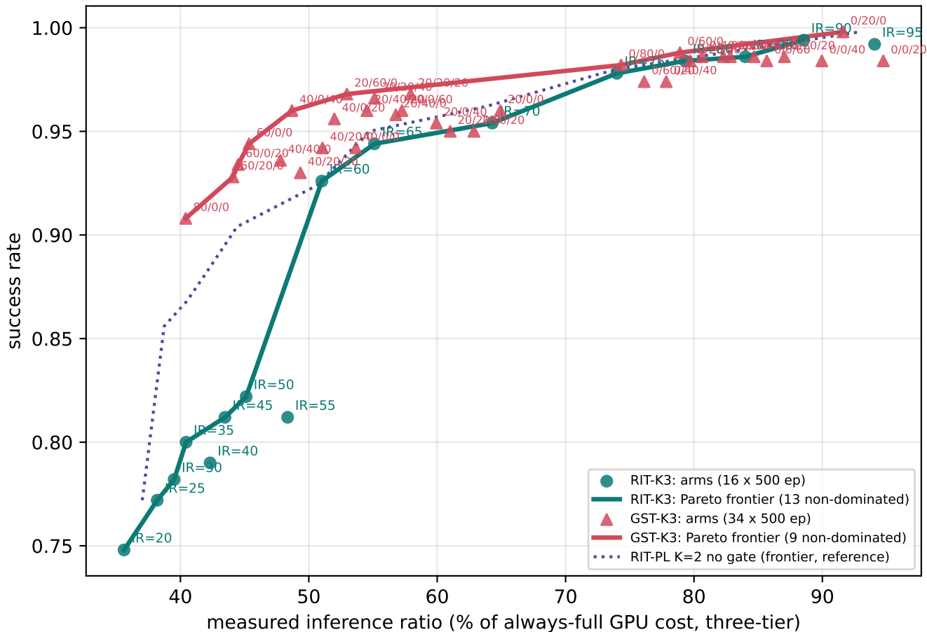
libero_spatial: K=3 ladder (FULL / WARM@0.3 / WARM@0.5), no gate, pruned-500 pool
