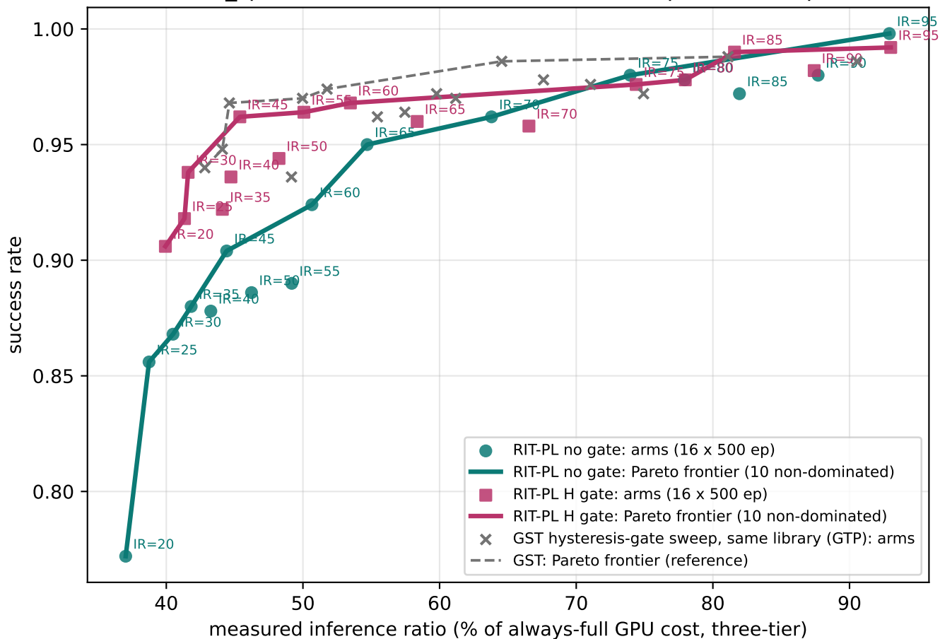
libero_spatial: RIT-PL frontiers on the official pruned-500 pool
