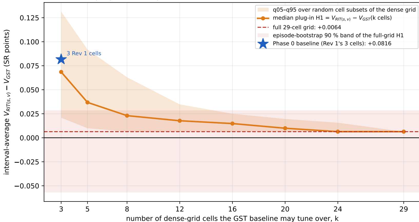
How RIT's margin shrinks with GST's tuning freedom (plug-in, development set; RIT(s,v) itself has only 3 measured arms)
