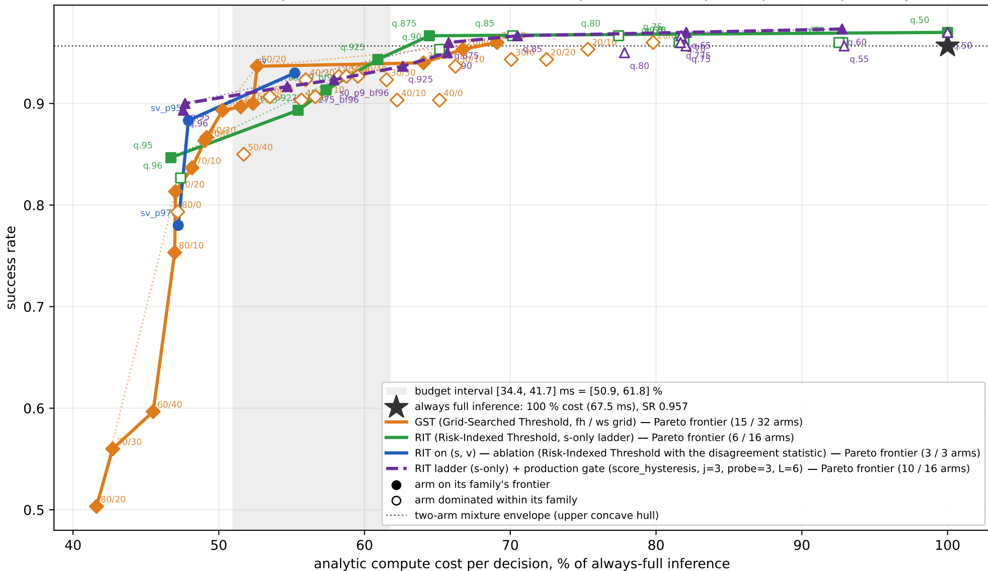
libero_spatial: measured arms by family — solid = per-family Pareto frontier, dotted = mixture envelope GST labels = fh/ws percentiles; RIT labels = calibration quantile (development points, exploratory)
