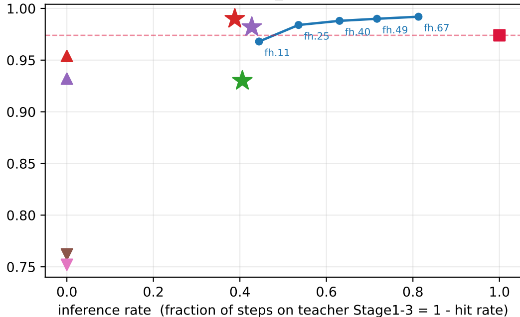
libero_spatial
