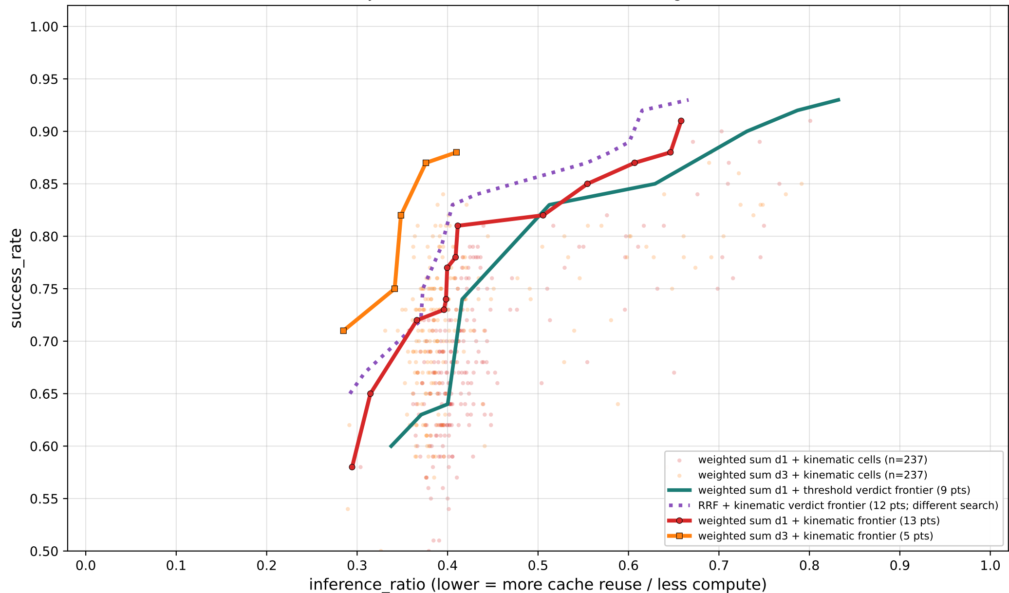
Pareto frontiers — search × verdict comparison on libero_10 No baseline / no always-warm anchors; colored scatter = all weighted-sum kinematic cells
