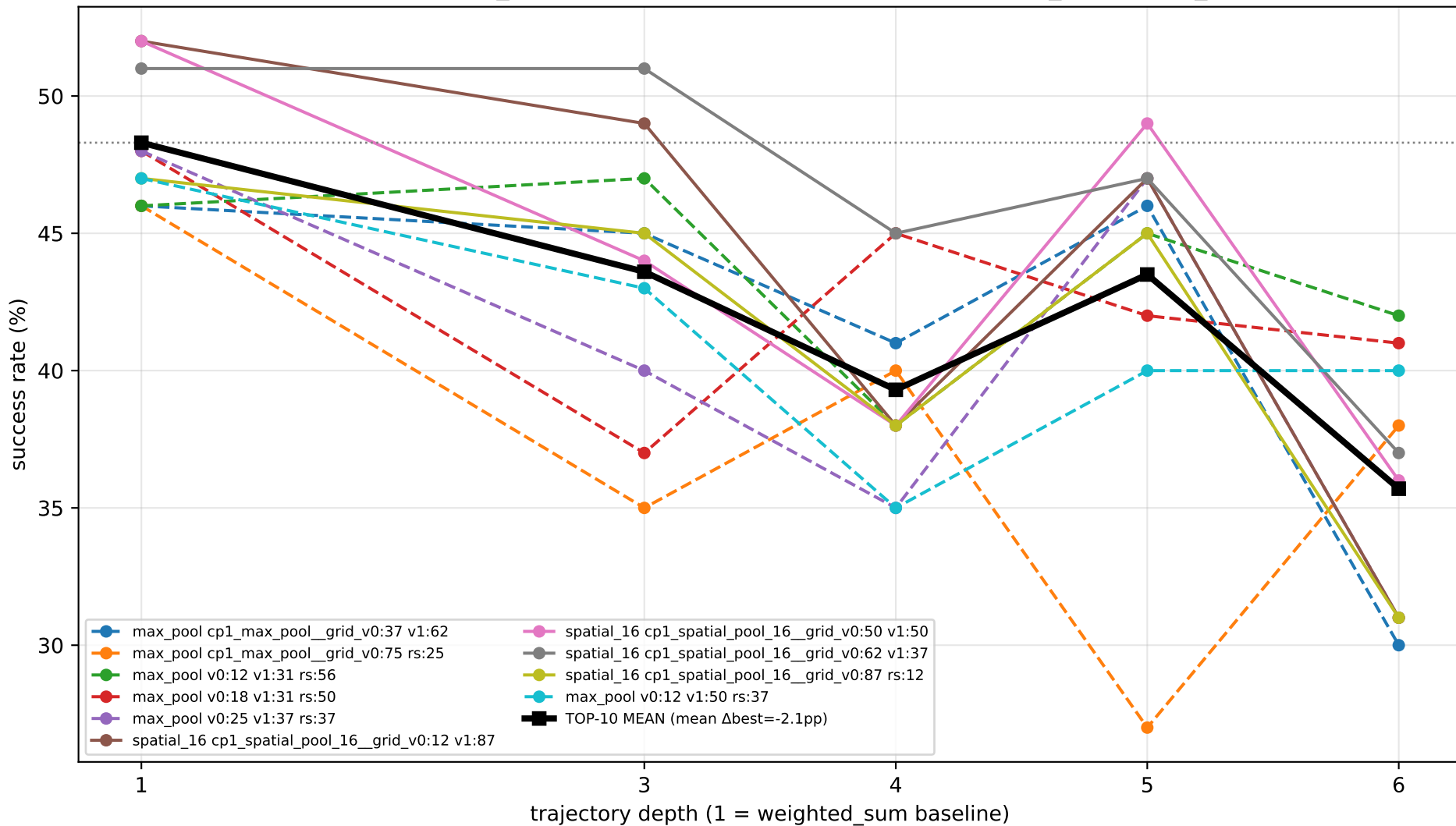
Top-10 weighted_sum configs under trajectory search (libero_10, always_hit)
