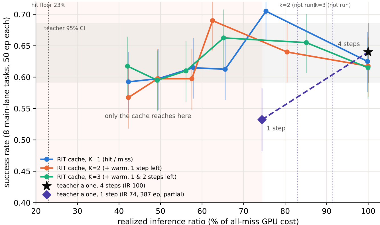
RoboCasa365 x GR00T N1.5: cache frontier vs fewer denoising steps (bars: Wilson 95% CI, 400 e
