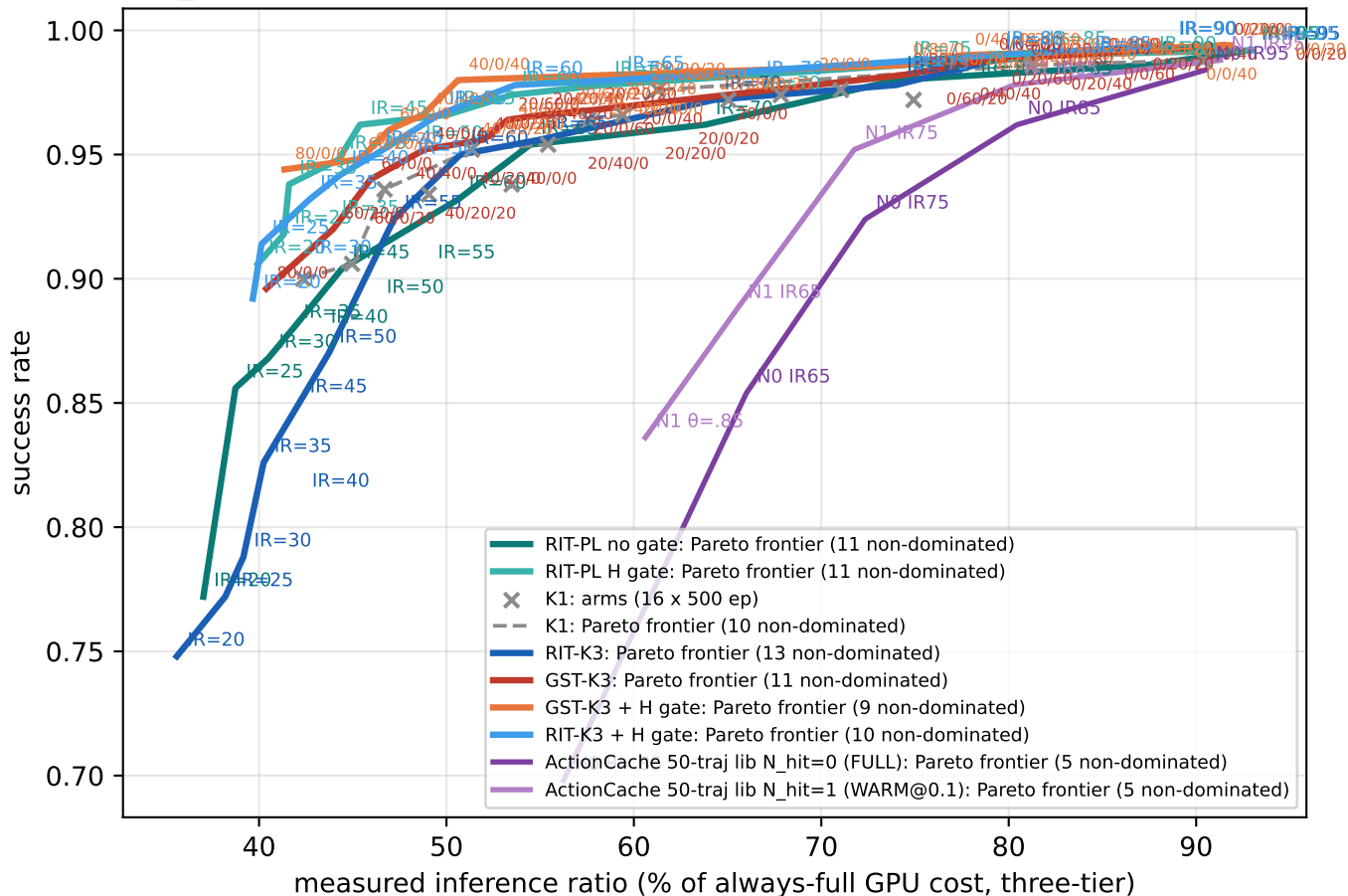
libero_spatial: RIT / GST / ActionCache frontiers on the official pruned-500 pool
