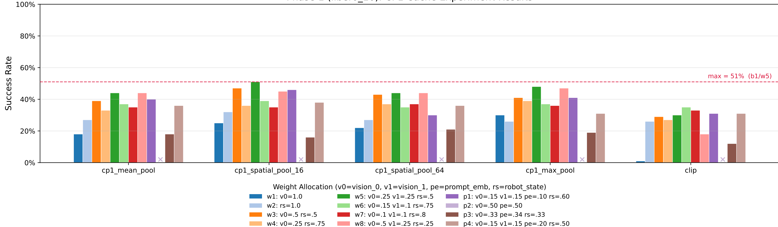
Phase 1 (libero_10): CP1 Cache Experiment Results
