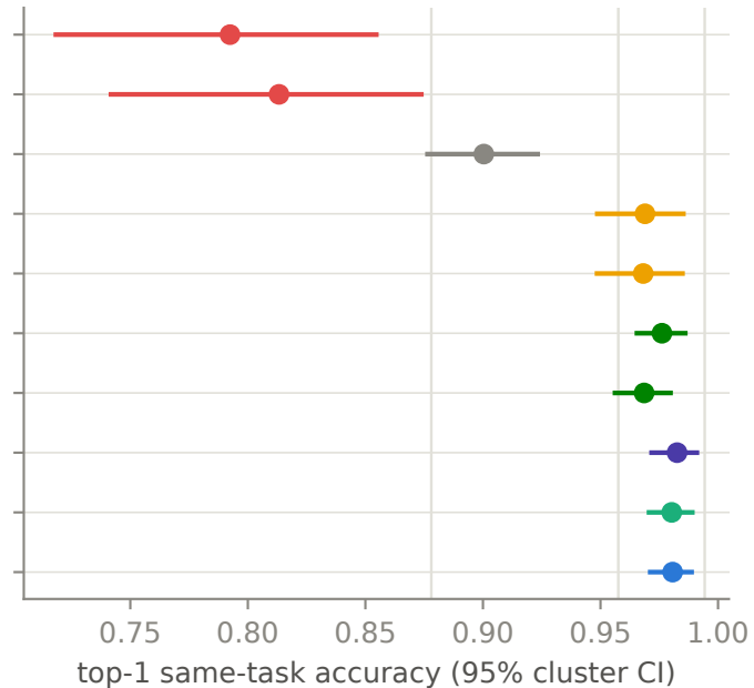
libero_10/cp1_spatial_pool_16
