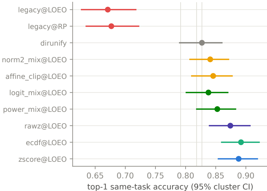
libero_spatial/cp1_spatial_pool_16
