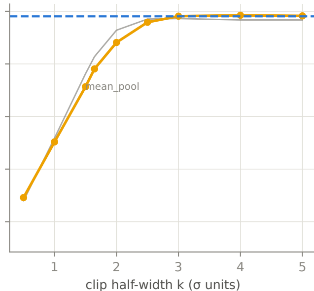
libero_10/cp1_spatial_pool_16
