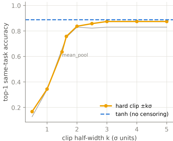
libero_spatial/cp1_spatial_pool_16
