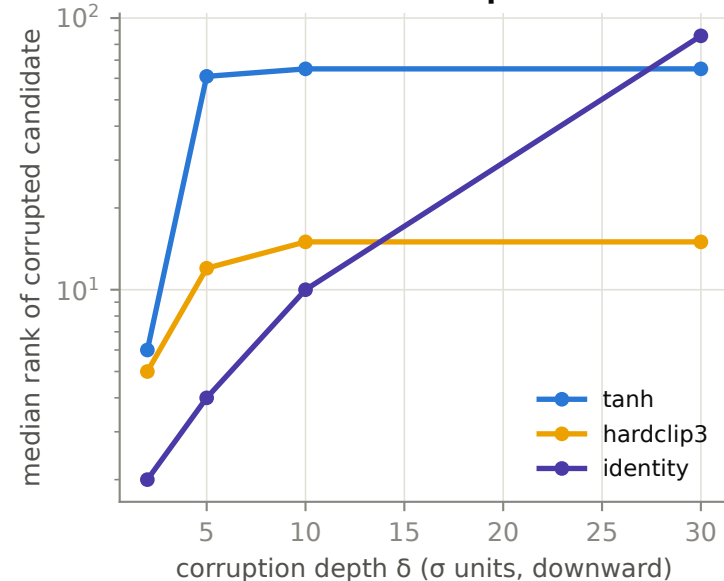
Bounded influence: rank plateaus vs sinks
