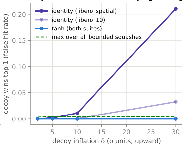
Decoy attack: unbounded maps get bought
