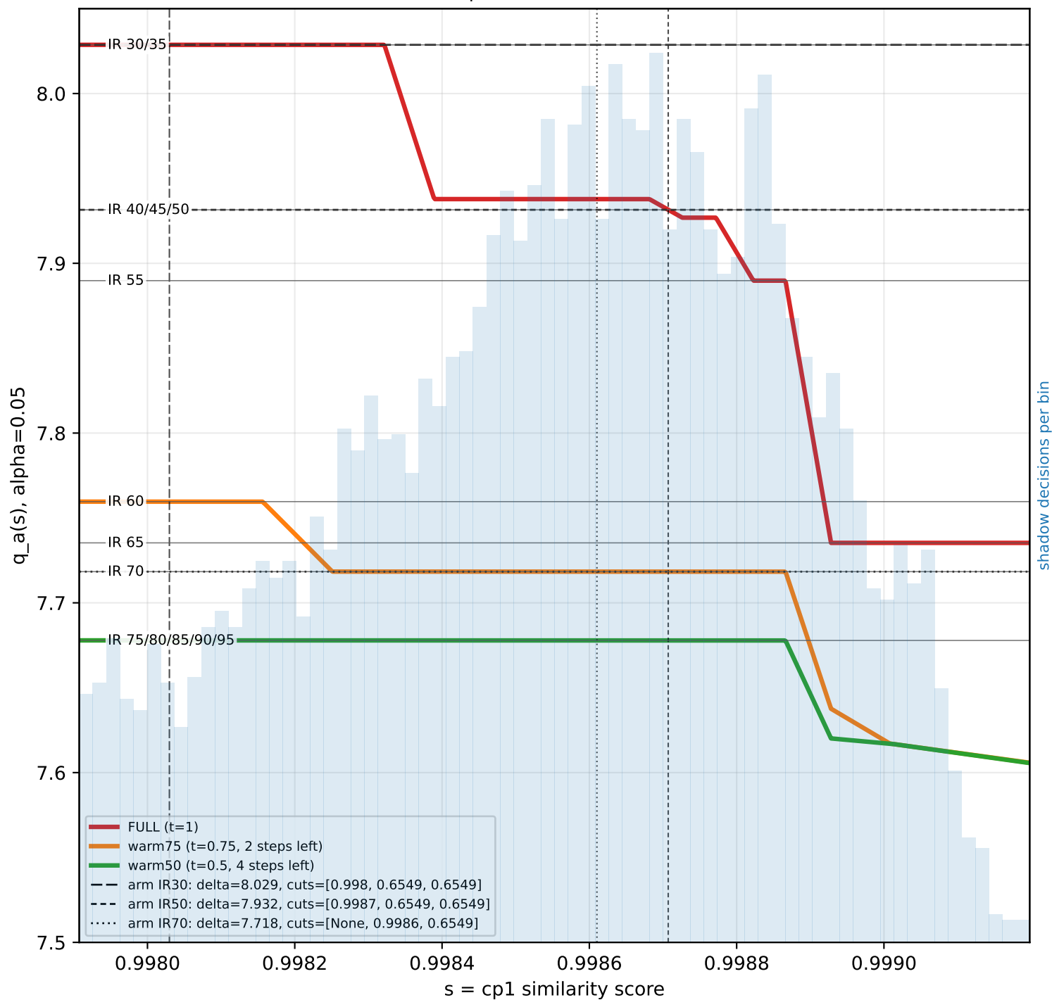
MAIN RUN libero_10 K=3 (shadow fit, n=8383) x in [25% quantile 0.9979, max 0.9992]
