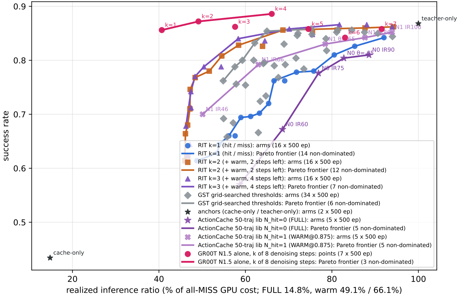
LIBERO-10: GR00T N1.5 warm-start cache, RIT ladder vs GST (500 episodes per arm)
