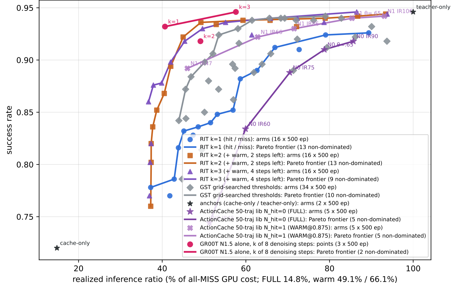
LIBERO-Spatial: GR00T N1.5 warm-start cache, RIT ladder vs GST (500 episodes per arm)
