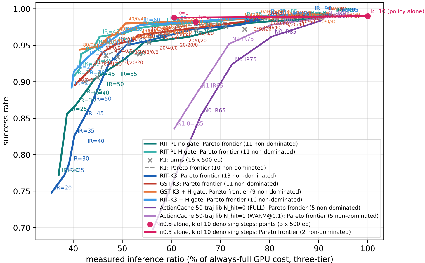
libero_spatial: RIT / GST / ActionCache frontiers on the official pruned-500 pool
