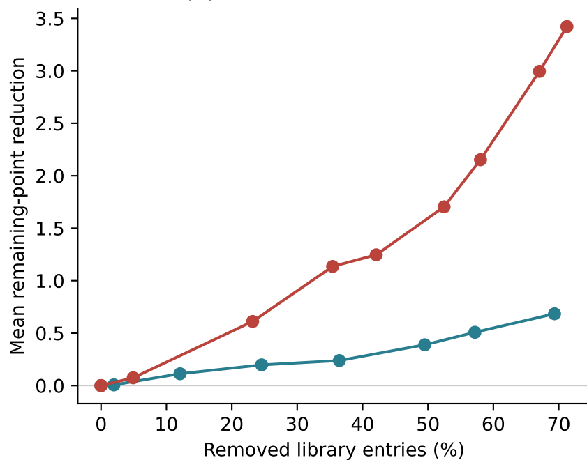
(b) Short-continuation bias
