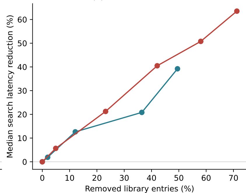
(c) Local CPU search
