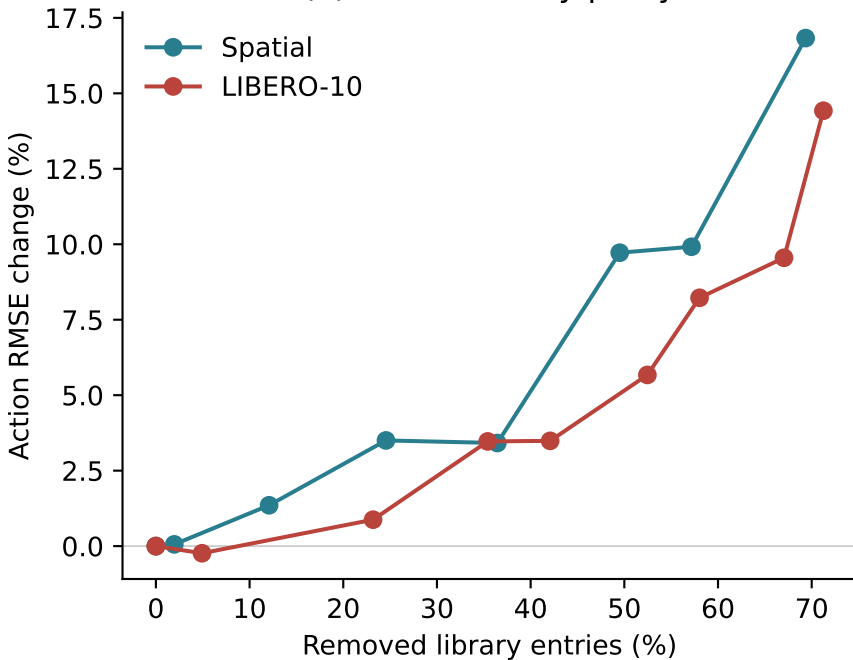
(a) Action fidelity proxy
