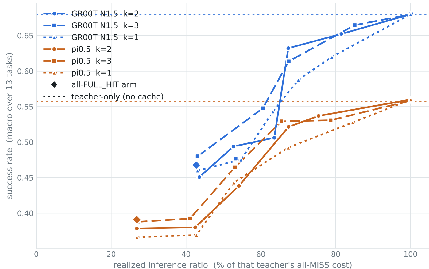
RoboCasa365 warm-start RIT frontier -- both teachers, 13 tasks x 50 episodes
