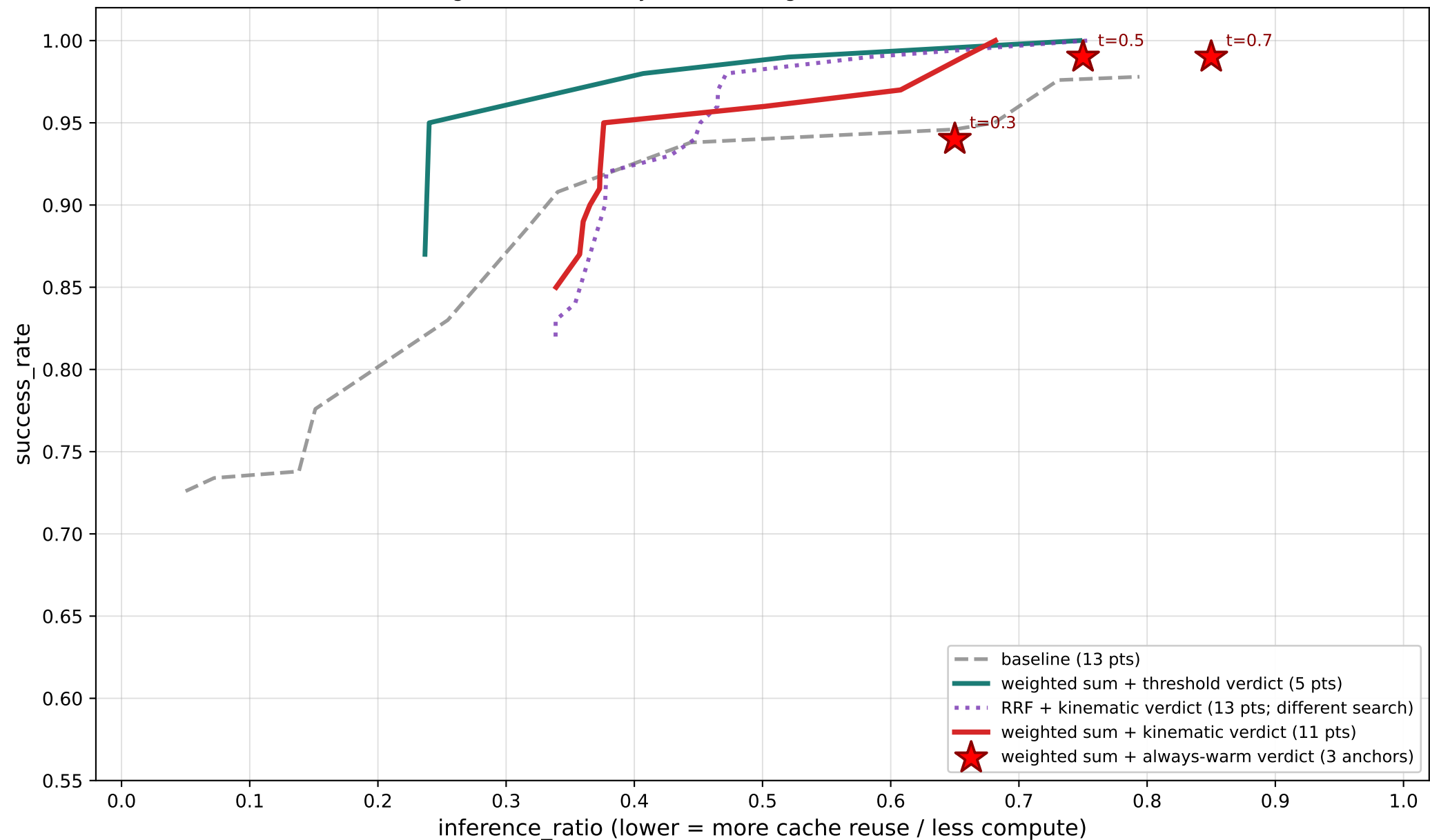
Pareto frontiers — search × verdict comparison on libero_spatial d1
