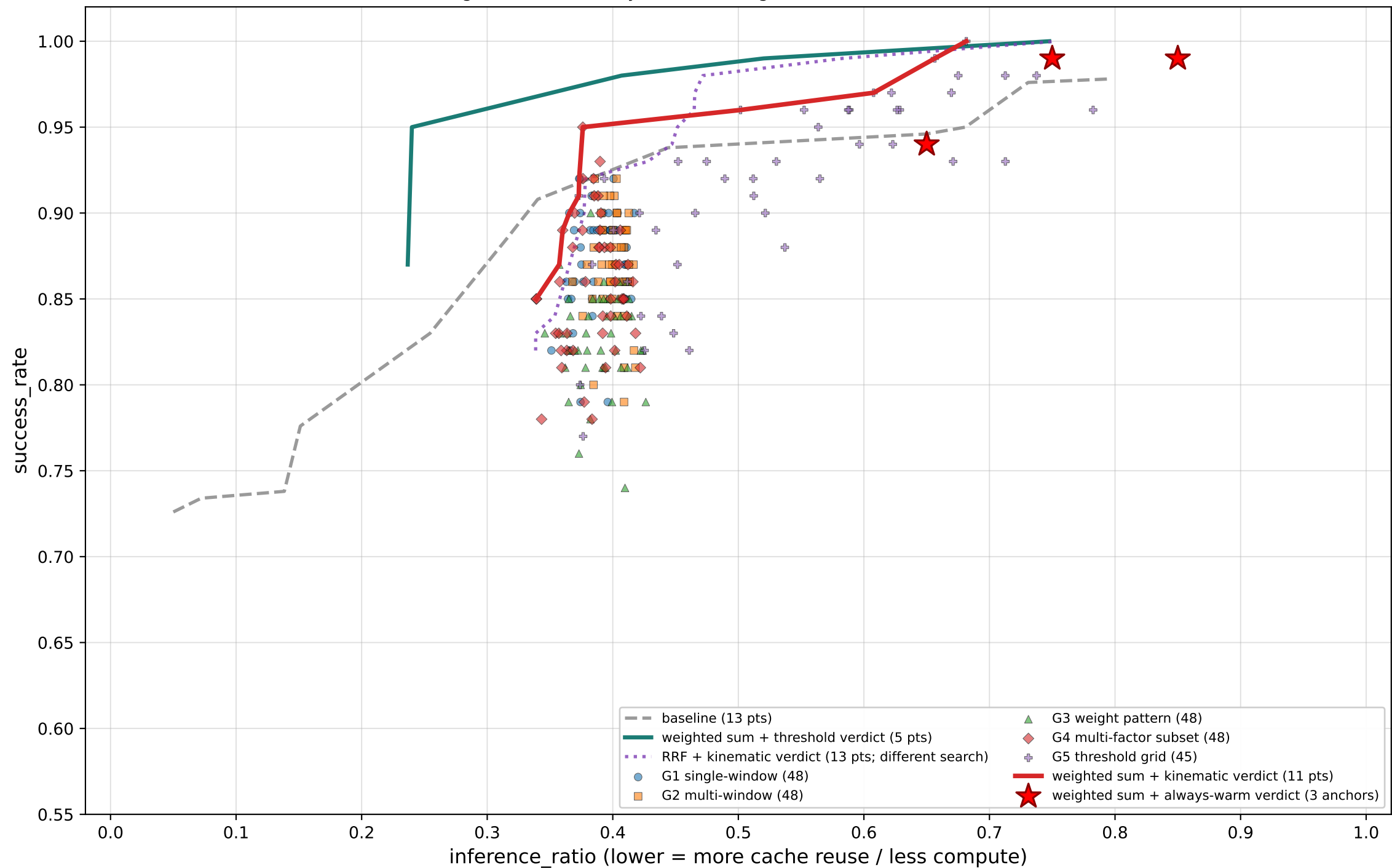
Pareto frontiers — search × verdict comparison on libero_spatial d1 ★ = self-measured weighted-sum + always-warm ceiling (RRF anchors NOT reused — cross-search invalid)
