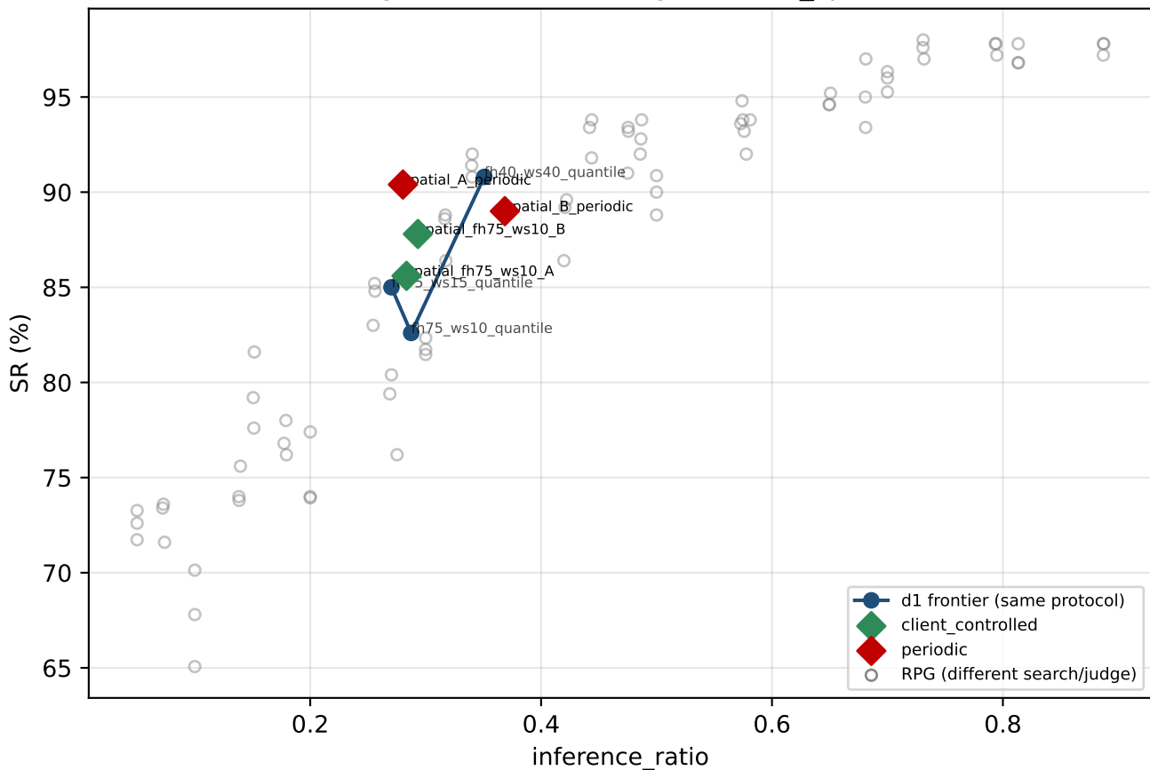
Stage 2b Pareto overlay — libero_spatial
