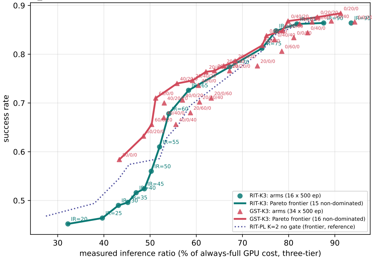
libero_10: K=3 ladder (FULL / WARM@0.3 / WARM@0.5), no gate, pruned-500 pool
