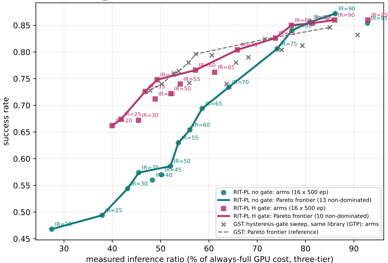
libero_10: RIT-PL frontiers on the official pruned-500 pool
