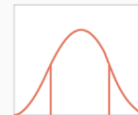
T-test distribution
