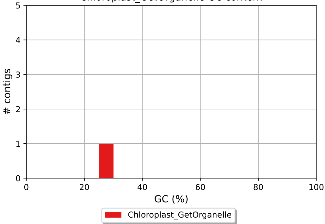
Chloroplast_GetOrganelle GC content
