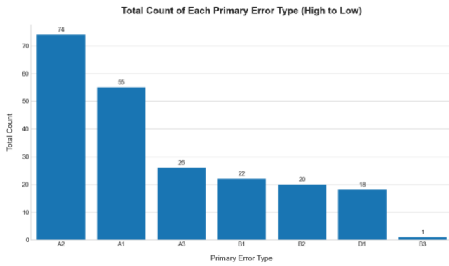
(a) DeepSeek error distribution
