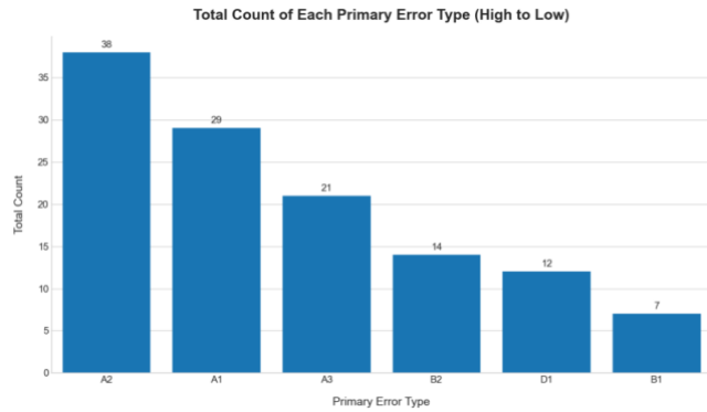
(b) Gemini error distribution
