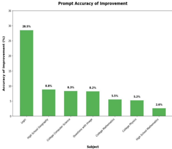
Fig. 2. Improvement gained by using different prompting strategies.
