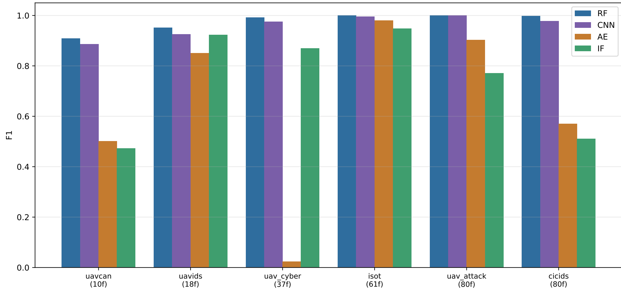
Detection Performance (F1)
