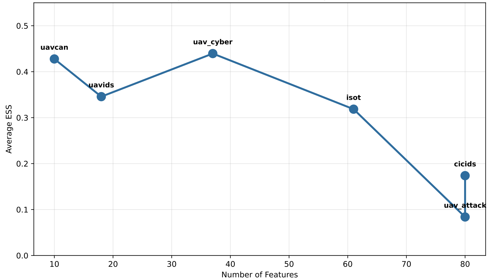
Stability Decreases with Dimensionality ( r=-0.85 )
