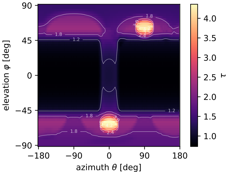
isocentre: \tau min 0.73, max 4.36
