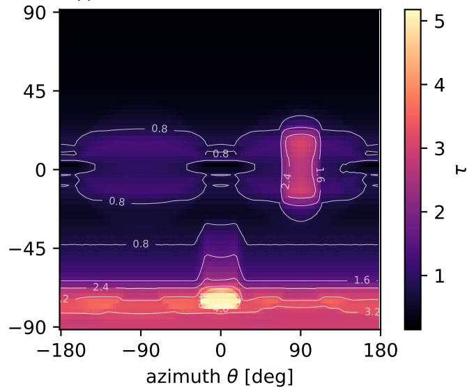
upper LoF stack: \tau min 0.15, max 5.18
