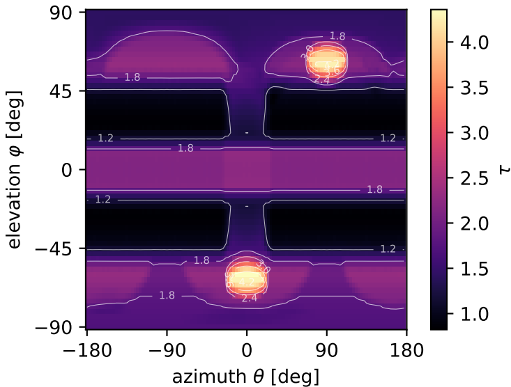
isocentre: \tau min 0.82, max 4.36
