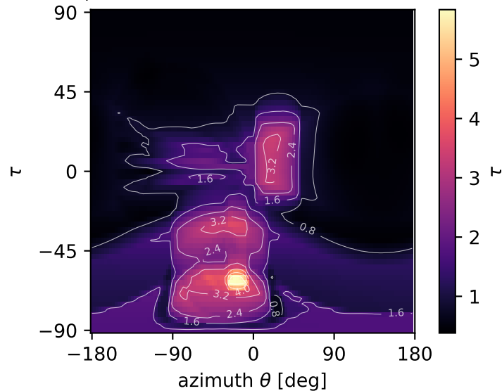
pores beside insert: \tau min 0.38, max 5.84
