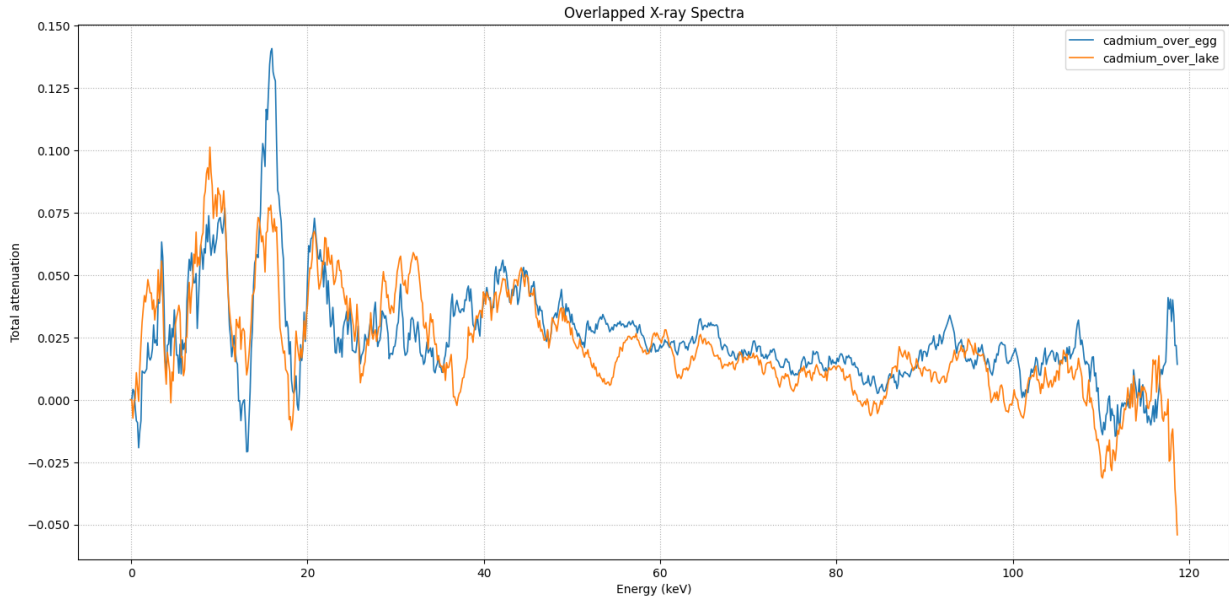
Figure 8: -\ln(I/I_0) signals for Cadmium Yellow, comparing the egg signal and the madder lake signal as I_0 The cadmium's K-edge (expected at 26.711\text{ keV} ) cannot be identified because of copper and aluminum X-ray filtration applied to the source.
