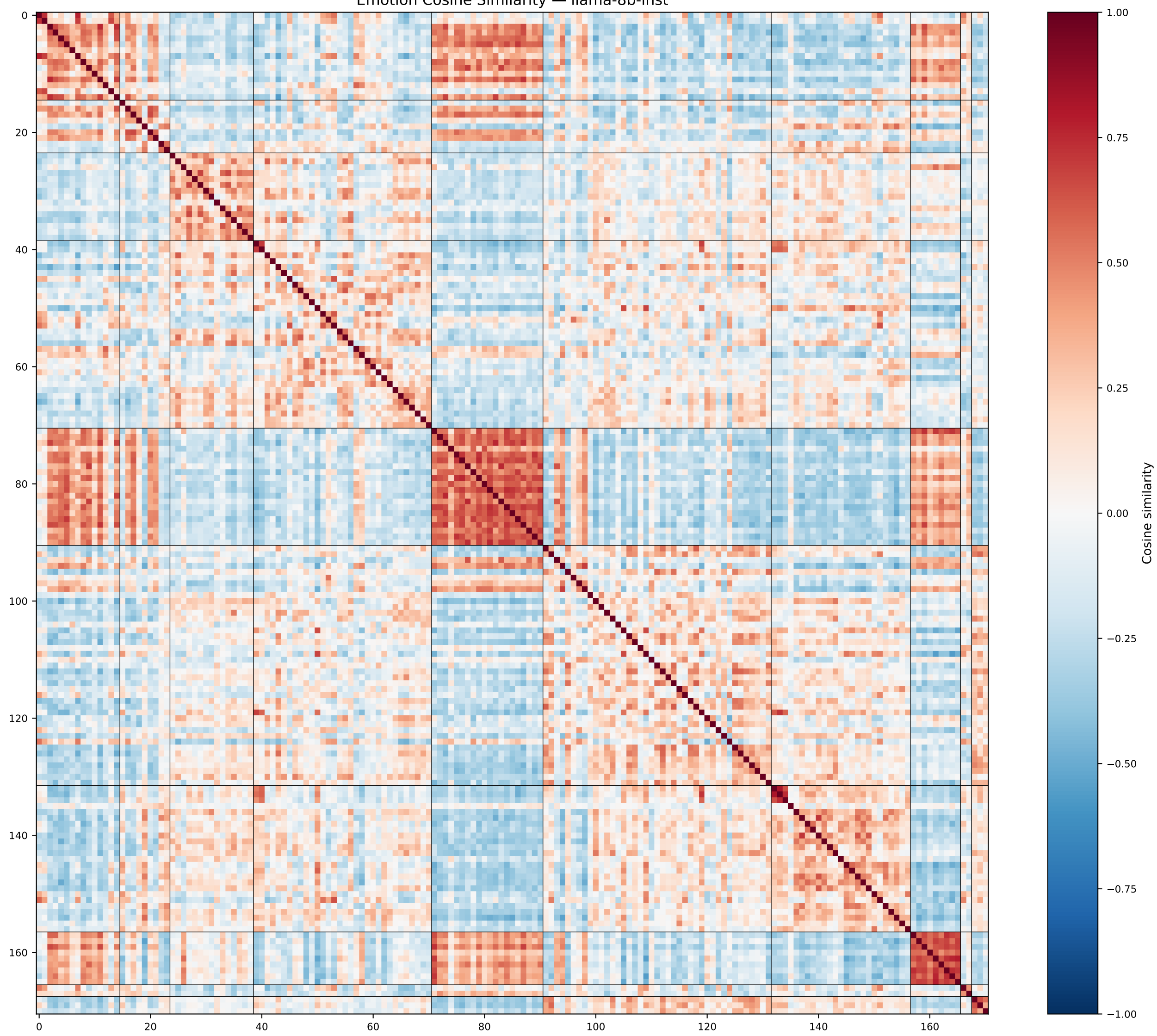
Emotion Cosine Similarity — llama-8b-inst
