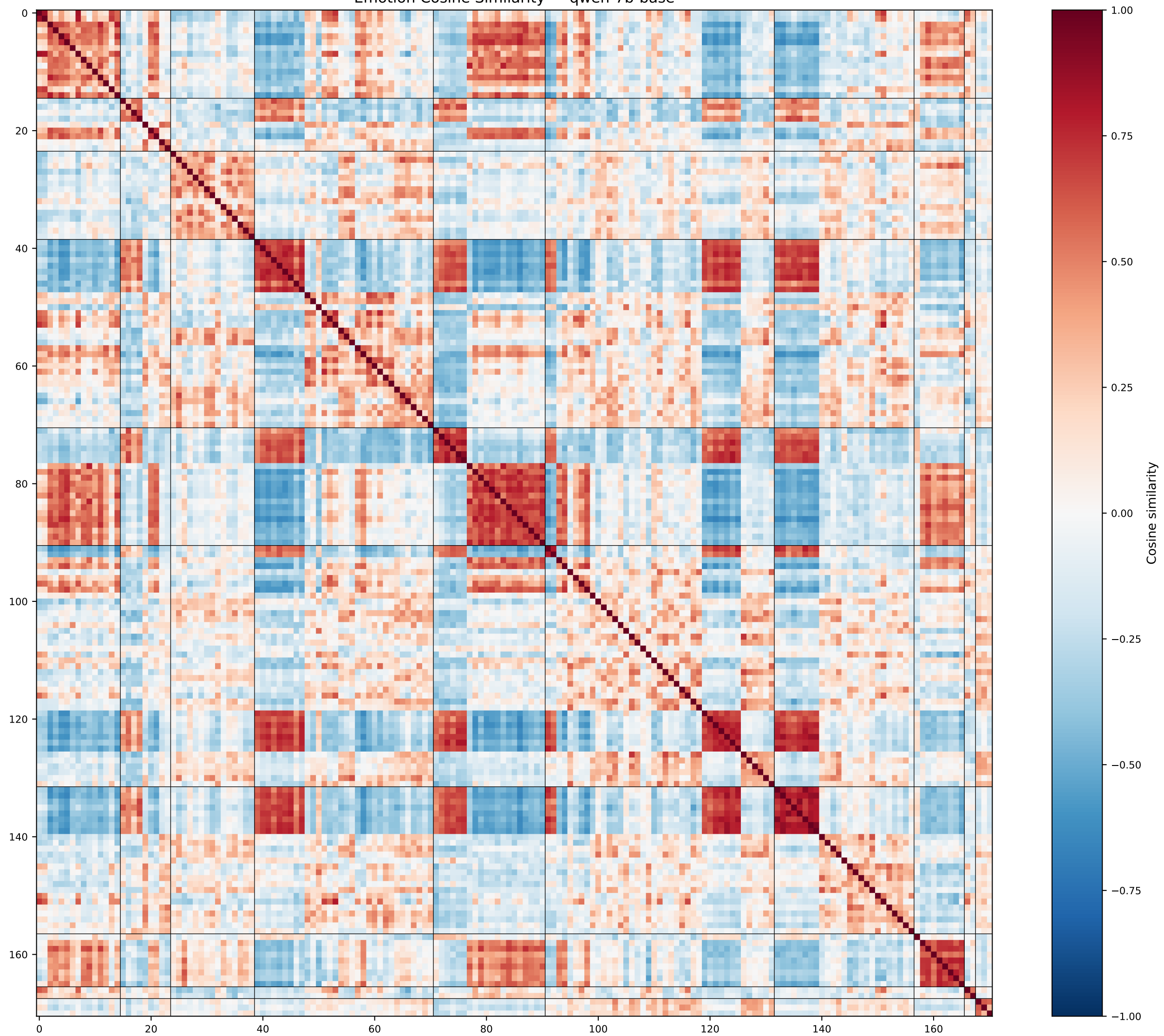
Emotion Cosine Similarity — qwen-7b-base
