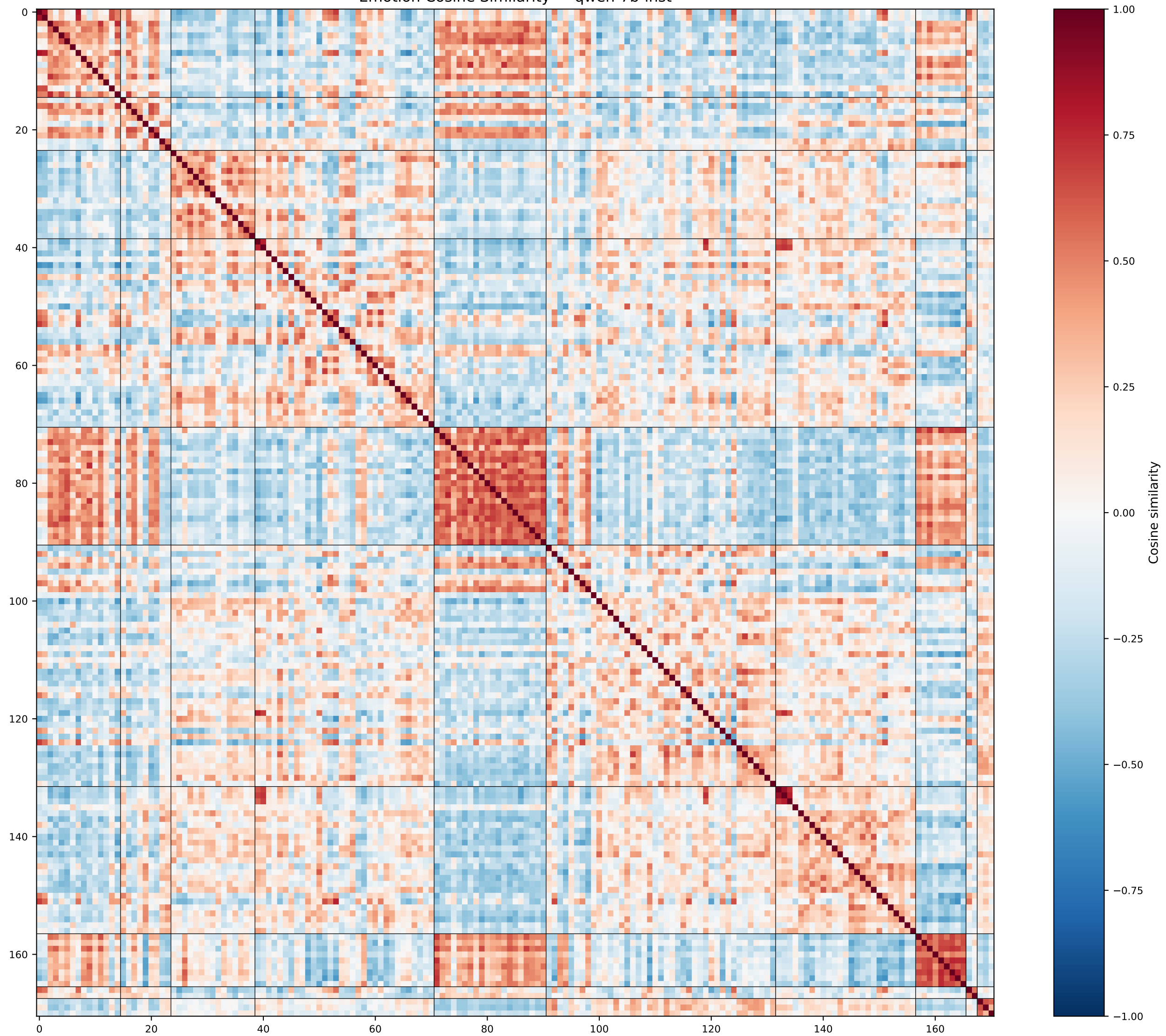
Emotion Cosine Similarity — qwen-7b-inst
