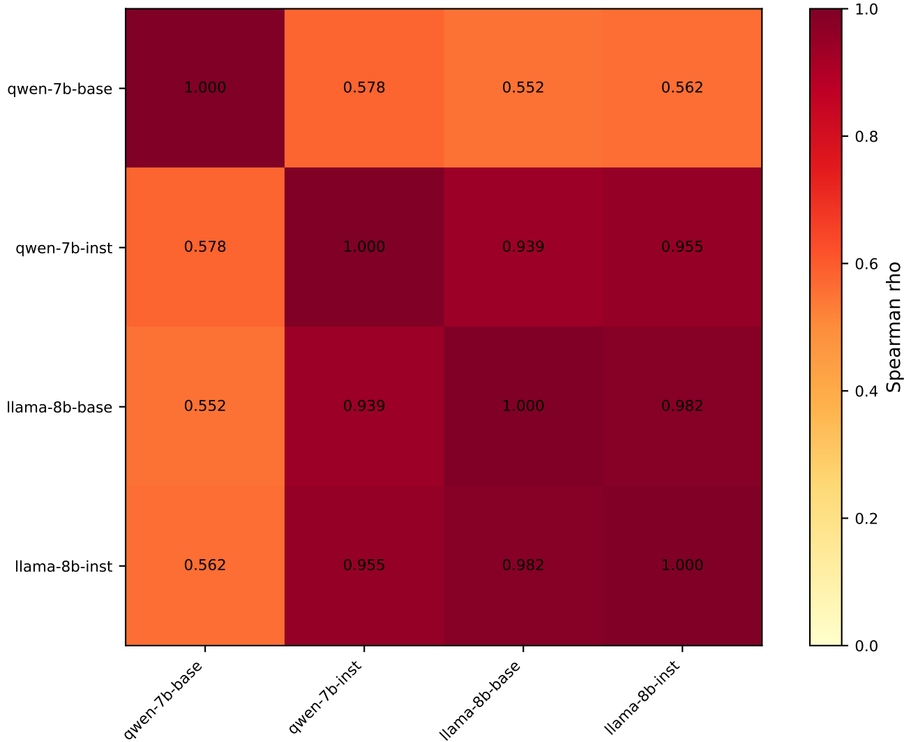
Cross-Architecture RSA
