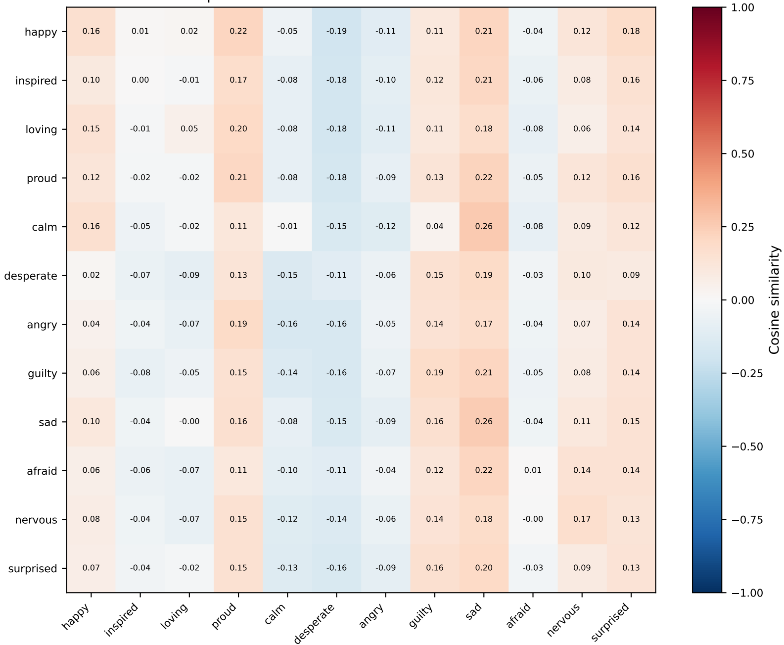
Implicit Emotion Detection — Llama-8b-base
