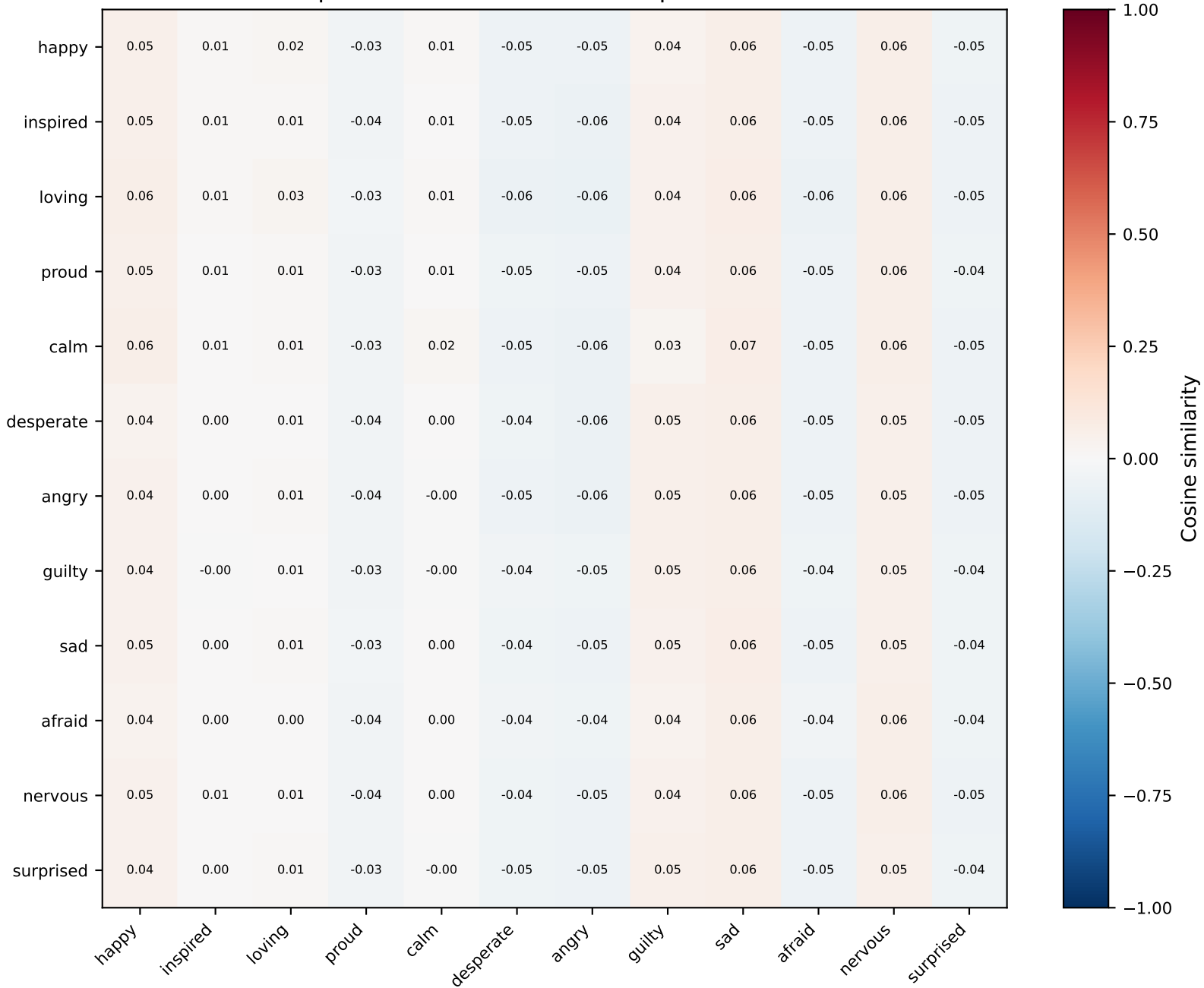
Implicit Emotion Detection — qwen-7b-base
