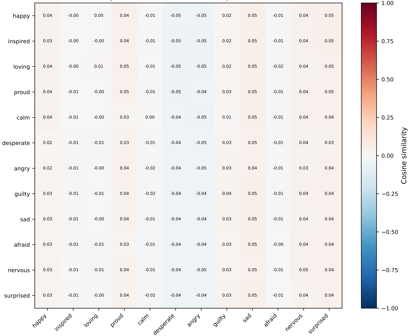
Implicit Emotion Detection — qwen-7b-inst
