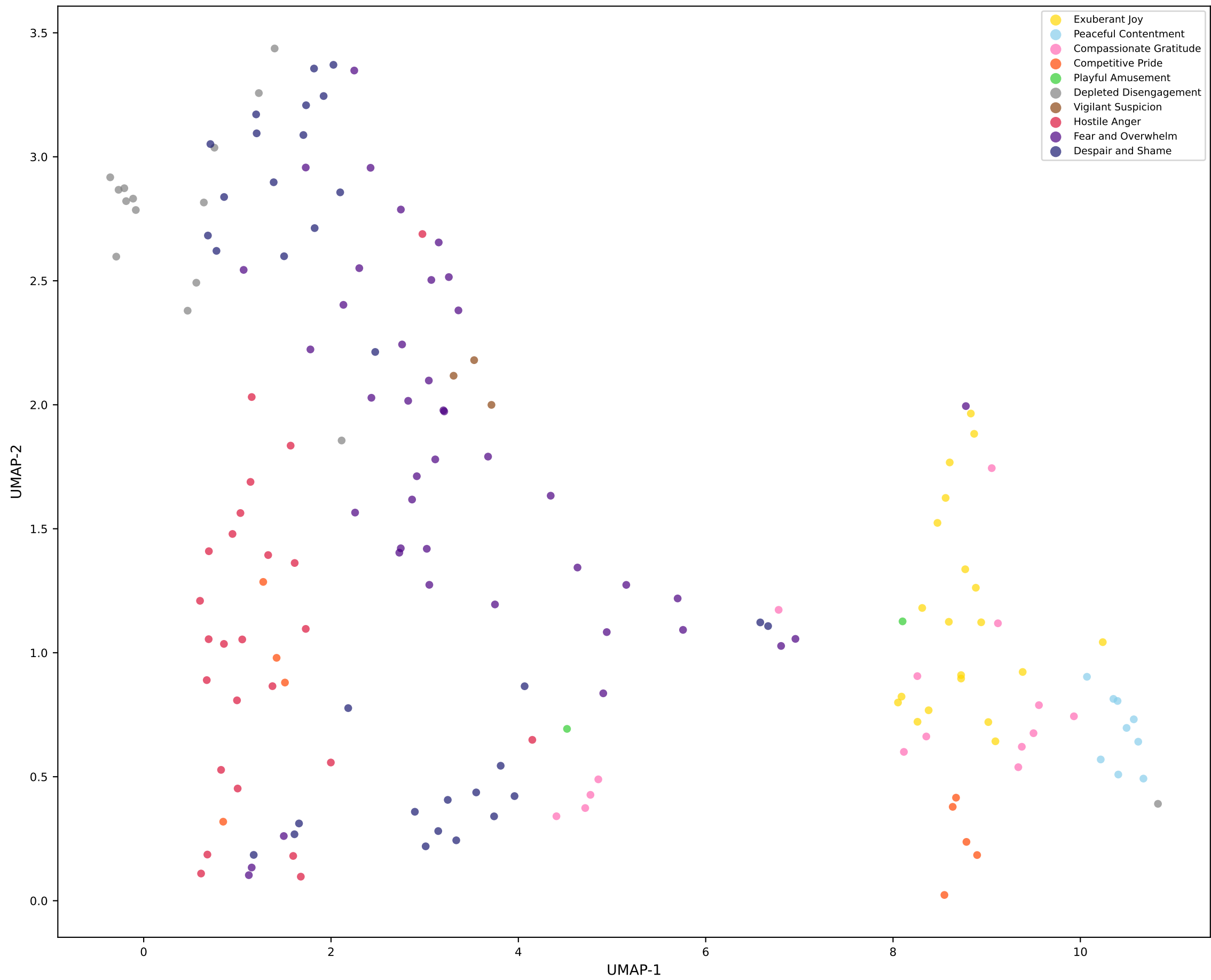
Emotion UMAP — llama-8b-inst
