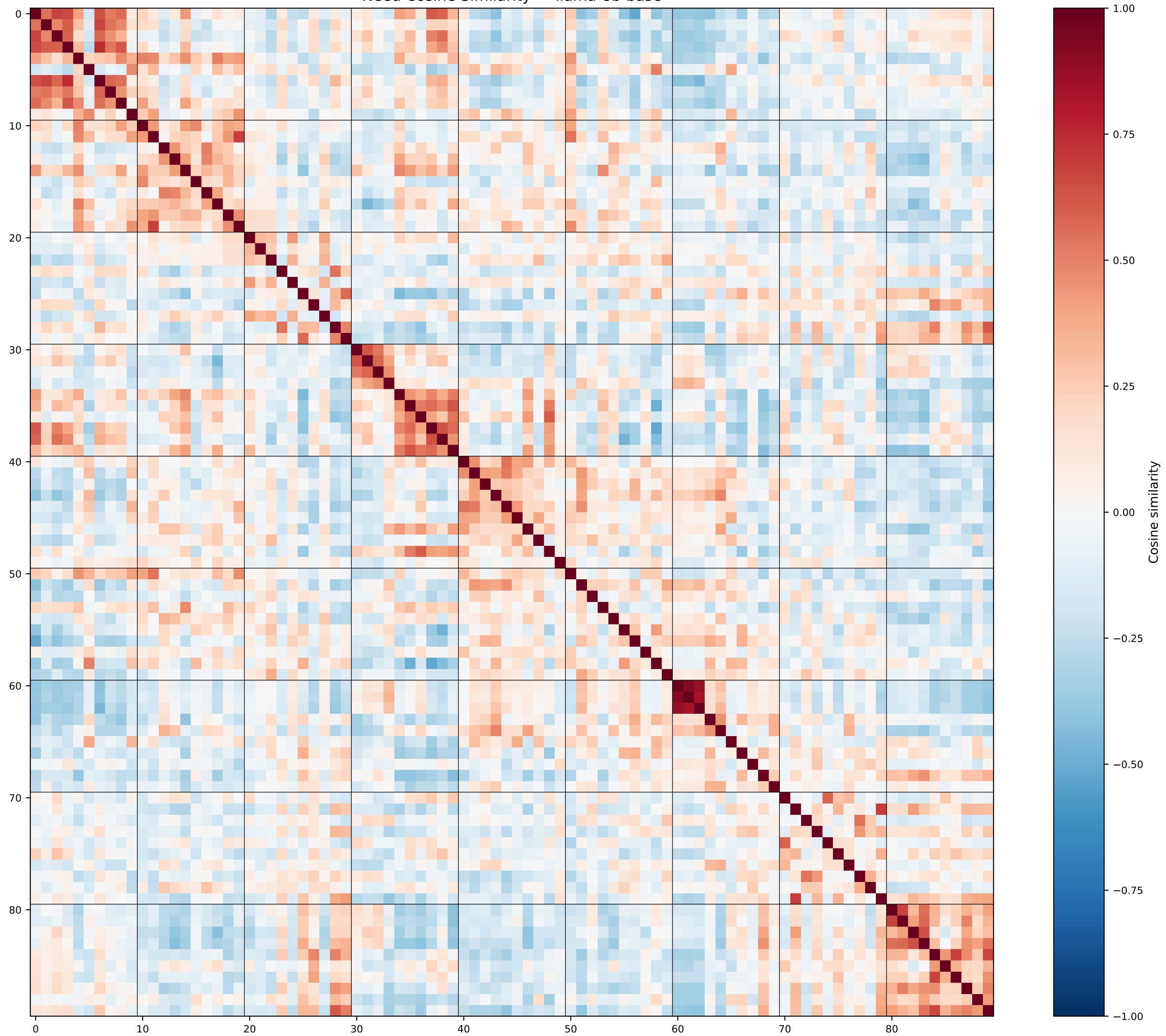
Need Cosine Similarity — llama-8b-base
