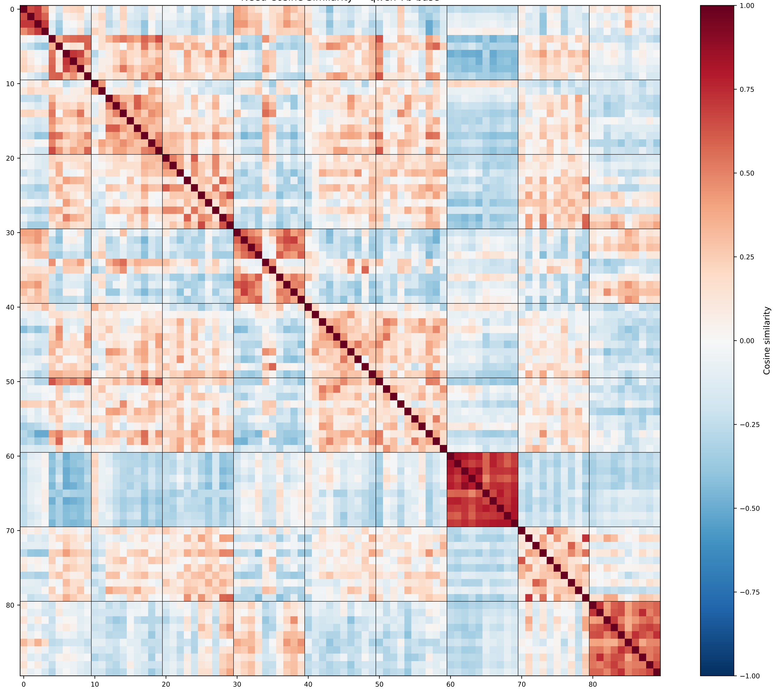
Need Cosine Similarity — qwen-7b-base
