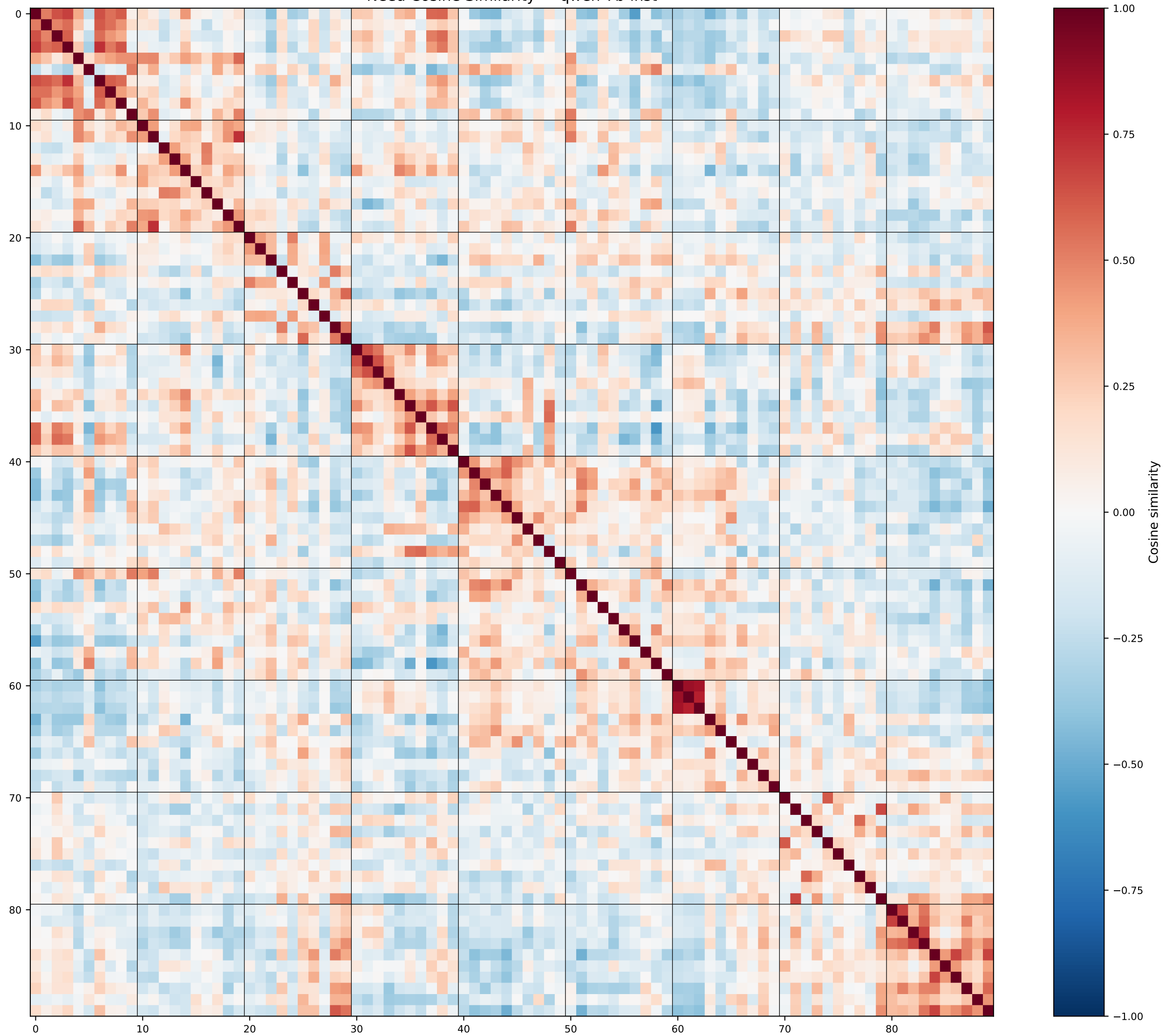
Need Cosine Similarity — qwen-7b-inst
