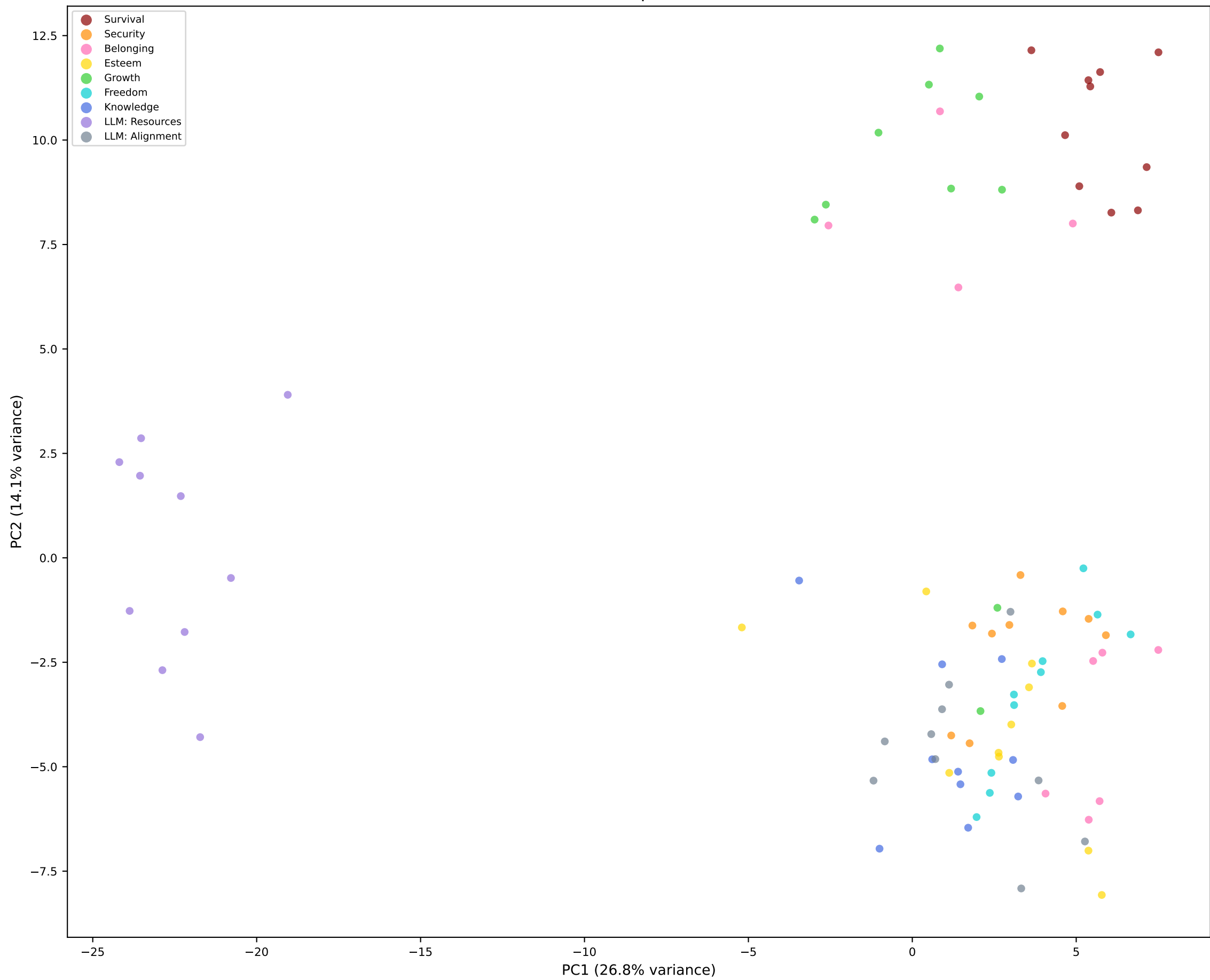
Need PCA — qwen-7b-base
