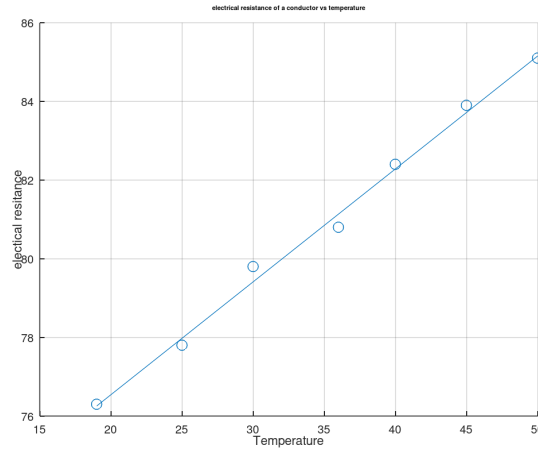
Figure 45: Visualization of linear regression (line): electrical resistance of a conductor as a function of temperature. —: regression line y = 0.28 \cdot x + 70.8 of the measurement X \mapsto Y with ○: (19, 25, 30, 36, 40, 45, 50) \mapsto (76.3, 77.8, 79.8, 80.8, 82.4, 83.9, 85.1) .
