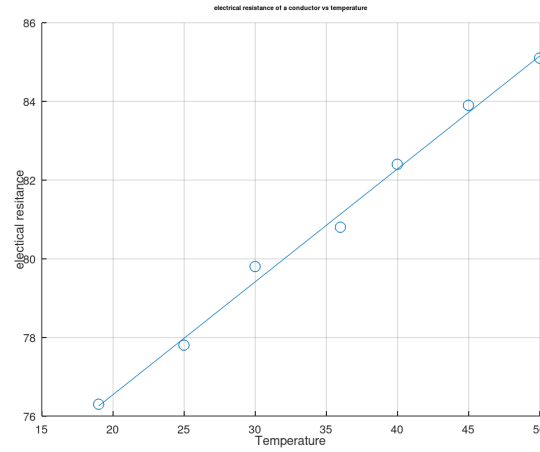
Figure 46: Visualization of linear regression (line): electrical resistance of a conductor as a function of temperature. —: regression line y = 0.28 \cdot x + 70.8 of the measurement X \mapsto Y with ○: (19, 25, 30, 36, 40, 45, 50) \mapsto (76.3, 77.8, 79.8, 80.8, 82.4, 83.9, 85.1) .
