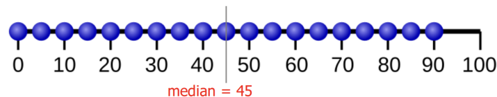
Figure 6: Figure illustrating the concept of median for the data set of the 19 numbers X = (0, 5, 10, \dots, 90) .
