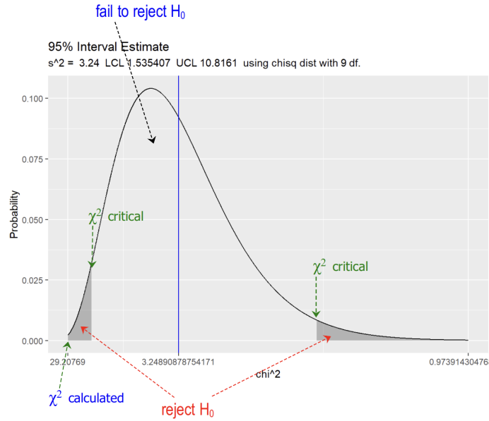
Figure 32: LCL = Lower Confidence Level; UCL = Upper CL; chisq = chi2INV . The values shown are from the solution of the example, see below.
