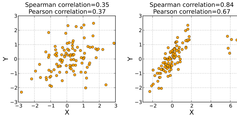
Figure 43: Visualization of SPEARMAN's rank coeff. \rho_S of two samples X and Y Left: For roughly elliptically distributed data with no prominent outliers, Spearman's \rho_S and Pearson's \rho correlation give similar values. Right: The Spearman correlation is less sensitive than Pearson's to strong outliers, because \rho_S limits the outlier to the value of its rank.
