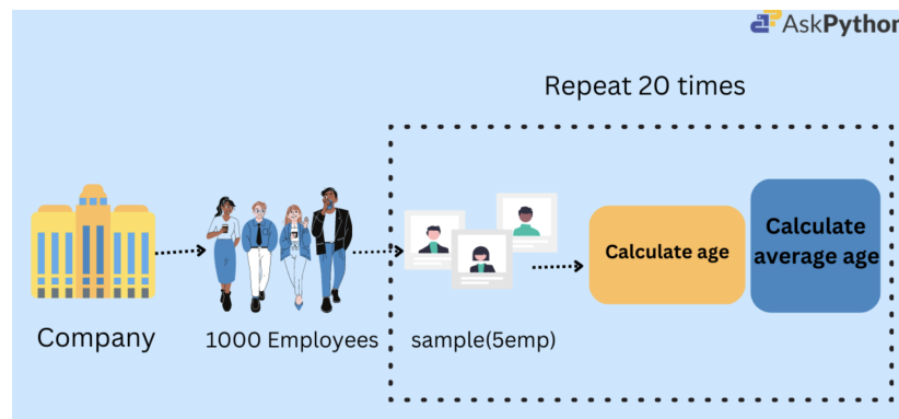
Figure 50: Visualization of bootCI : Instead of taking multiple samples directly from the whole employees population, we only draw a single, representative sample (5emp). We then generate e.g. 20 'new' samples by repeatedly create new bootstrap samples of the same size.
