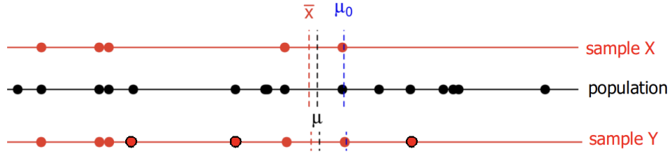
Visualization of Z-test for a Hypothesized Mean \mu_0 : Figure 28: \bullet : samples X and Y with sample means \bar{X} resp. \bar{Y} \bullet : population with population mean \mu .
