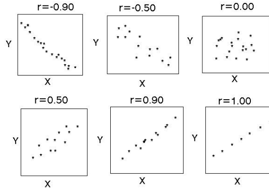
Figure 42: Visualization of PEARSON's correlation coefficient \rho : 6 typical cases. row1: from strong negative correlation ('-0.9') until no correlation ('0'). row2: from mean positive correlation ('+0.5') until strong positive correlation ('+1').
