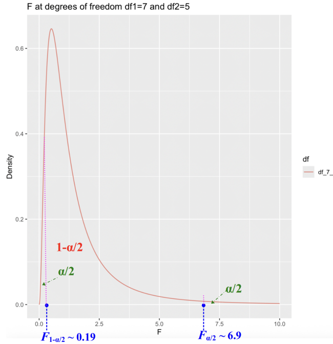
Figure 33: The values shown are from the solution of the example, see below.
