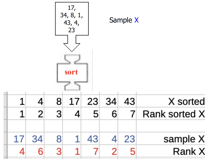
Figure 38: 1: X = (17, 34, 8, 1, 43, 4, 23) \xrightarrow{\text{sort}} (1, 4, 8, 17, 23, 34, 43) = X_{\text{sorted}} . 2: X_{\text{sorted}} = (1, 4, 8, 17, 23, 34, 43) \xrightarrow{\text{Rank}} (1, 2, 3, 4, 5, 6, 7) = X_{\text{ranked}} .
