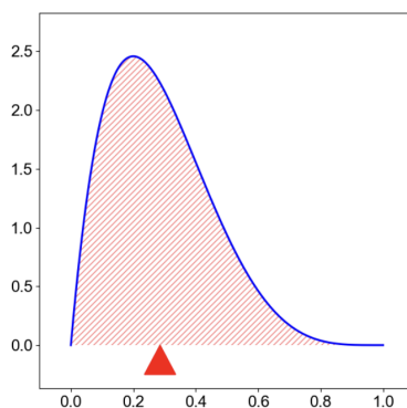
Imagine the data distributed under the blue graph. Then the moment Figure 9: may be interpreted as 'center of mass', balanced upon the 'expected' value \triangle , the moment e.g. the mean; Cf. GUNDERSEN
