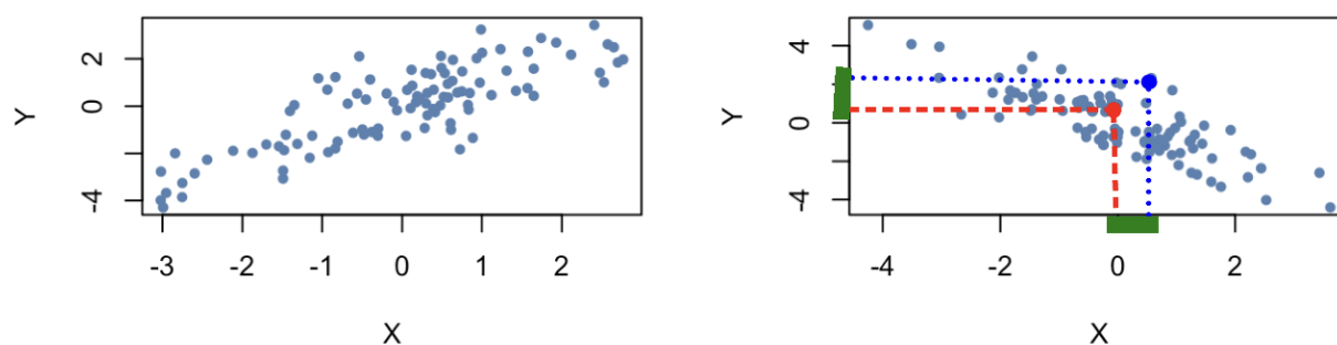
Figure illustrating the concept of covariance for a set of numbers. Left: Figure 12: positive cov. Right: negative cov. \bullet = (\bar{X}, \bar{Y}) . \bullet = (x_i, y_i) a data point. \text{green rectangle} = (x_i - \bar{X}) \cdot (y_i - \bar{Y}) a distance product w.r.t. the mean.
