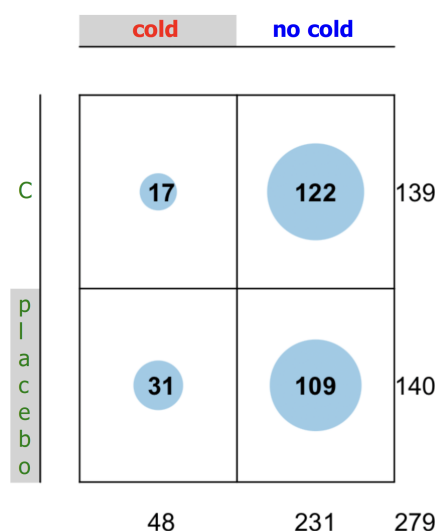
Figure 39: Visualization of Four-field Table for an experimental outcome. ●: experiment outcome as frequency table T = \begin{pmatrix} a & b \\ c & d \end{pmatrix} = \begin{pmatrix} 17 & 122 \\ 31 & 109 \end{pmatrix} .
