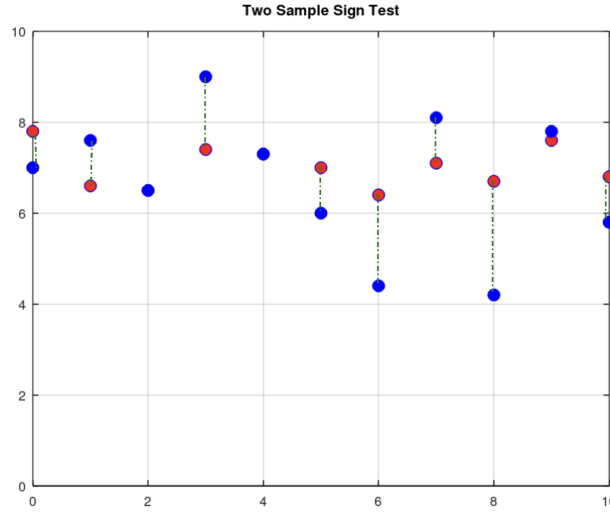
Figure 35: Visualization of sign2 -test on two samples X and Y with d_i = x_i - y_i . ●: sample X = (7.8, 6.6, 6.5, 7.4, 7.3, 7.0, 6.4, 7.1, 6.7, 7.6, 6.8) . ●: sample Y = (7.0, 7.6, 6.5, 9.0, 7.3, 6.0, 4.4, 8.1, 4.2, 7.8, 5.8) .
