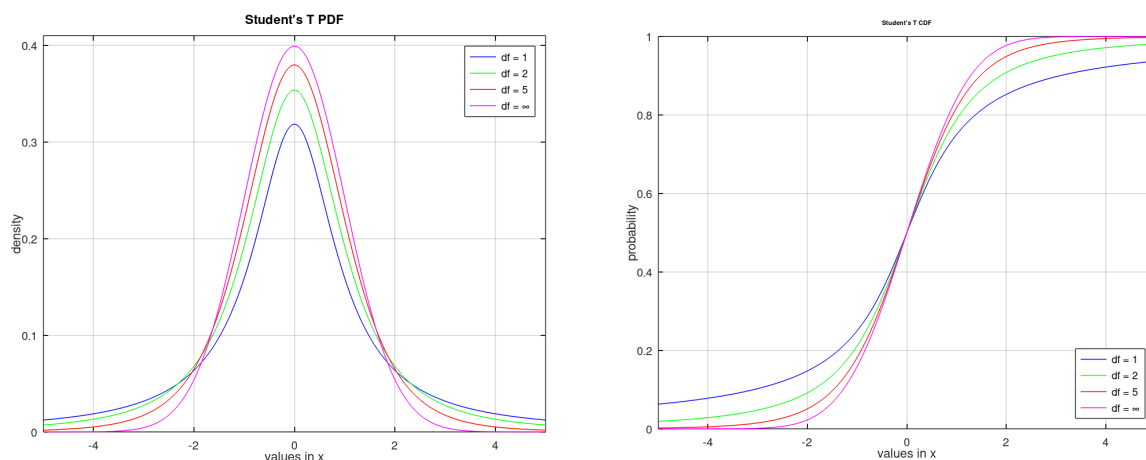
Figure 20: Student's t distributions with different degrees of freedom df := \nu . Left figure: \lambda = plot of \mathbf{tPDF}(x, \nu) , \nu = 1; 2; 5 . Check \mathbf{tPDF}(0, 1) = 0.3 on the graph. Right figure: \lambda = plot of \mathbf{tCDF}(x, \nu) , \nu = 1; 2; 5 . Check \mathbf{tCDF}(0, 1) \approx 0.5 on the graph. Check \mathbf{tINV}(0.2, 1) \approx -1 on the CDF via y = 0.2 \rightarrow \downarrow -1 = x
