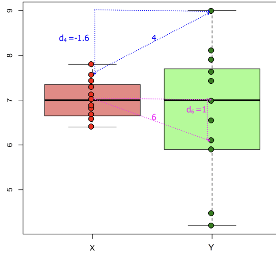
Figure 37: Visualization of Two Sample WILCOXON-test on two samples X and Y ●: sample X = (7.8, 6.6, 6.5, 7.4, 7.3, 7.0, 6.4, 7.1, 6.7, 7.6, 6.8) . ●: sample Y = (7.0, 7.6, 6.5, 9.0, 7.3, 6.0, 4.4, 8.1, 4.2, 7.8, 5.8) . ●: For pair 6 we have d_6 = x_6 - y_6 = 7 - 6 = +1 .
