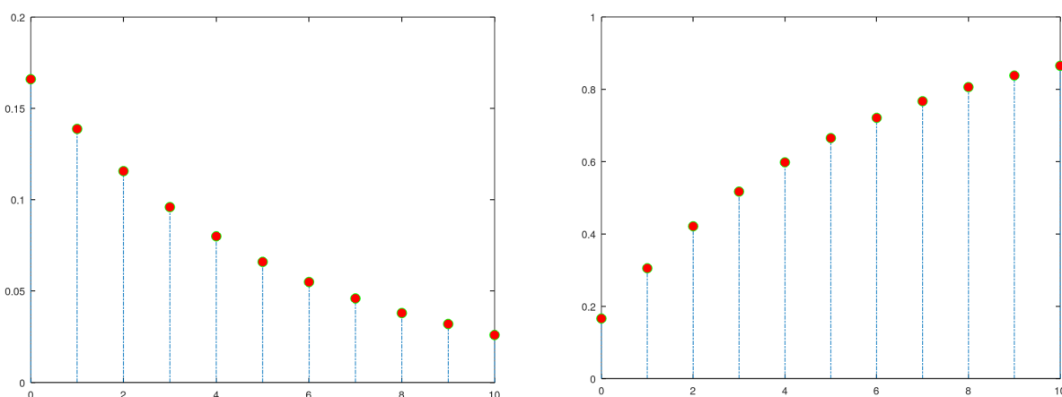
Figure 14: Experiment: rolling a six-sided die. Left figure: \bullet = plot for \text{geoPDF}(k, 1/6) for k = 0, \dots, 10 . Check \text{geoPDF}(4, 1/6) = 0.08 on the graph. Right figure: \bullet = plot for \text{geoCDF}(k, 1/6) for k = 0, \dots, 10 . Check \text{geoCDF}(5, 1/6) = 0.665 on graph. Check \text{geoINV}(0.7, 1/6) = 6 on the CDF graph via y = 0.6 \rightarrow \downarrow 6 = k
