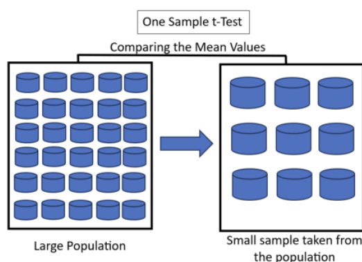
Figure 29: Visualization of one-sample- t -test for a hypothesized mean \mu_0 : ▷ wiki
