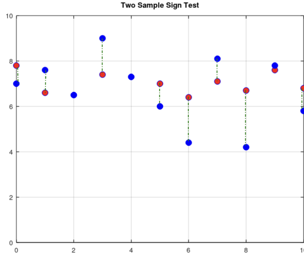
Figure 34: Visualization of sign2 -test on two samples X and Y with d_i = x_i - y_i . ●: sample X = (7.8, 6.6, 6.5, 7.4, 7.3, 7.0, 6.4, 7.1, 6.7, 7.6, 6.8) . ●: sample Y = (7.0, 7.6, 6.5, 9.0, 7.3, 6.0, 4.4, 8.1, 4.2, 7.8, 5.8) .
