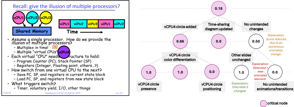
Figure 6. Example rubric tree and scores for the “add vCPU4” task from Fig 1: critical and non-critical check scores and explanations aggregate to a graded outcome with overall explanatory text. The rubric correctly identifies and accordingly awards partial progress a vCPU4 circle but not positioning it correctly nor updating the time-sharing diagram.
