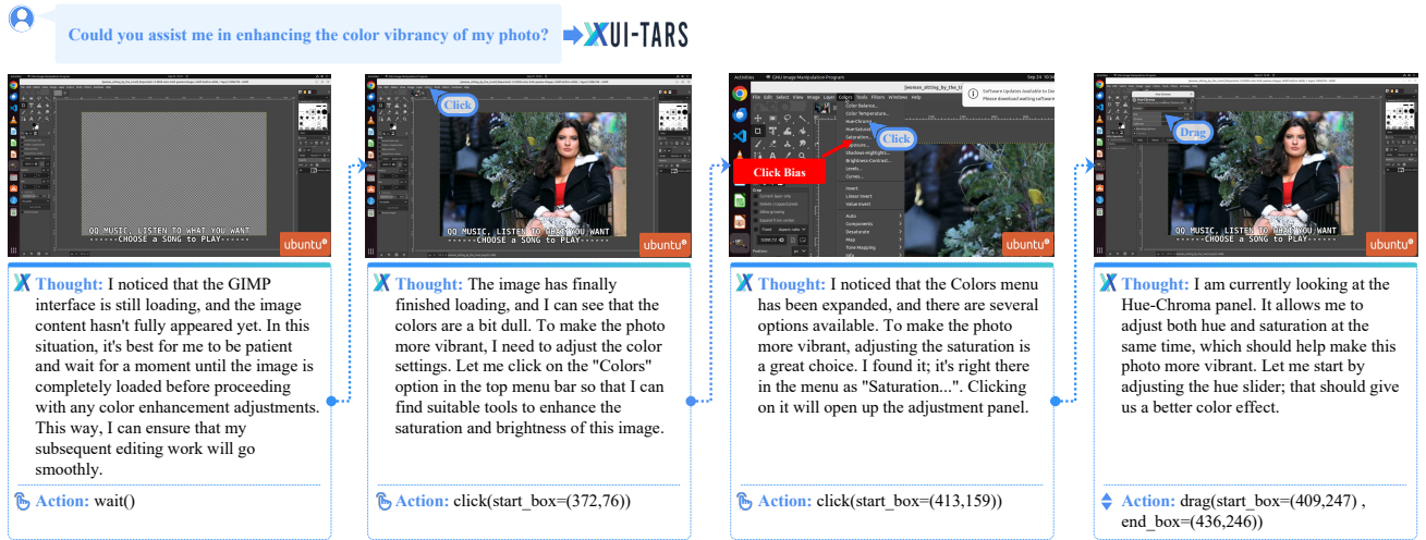
Figure 13. The performance of UI-TARS-1.5-7B when facing subtitle. The click positions deviate from the target positions.
