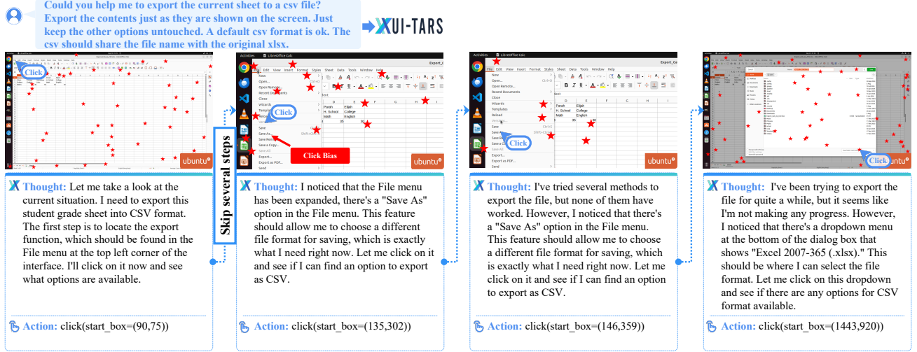
Figure 12. The performance of UI-TARS-1.5-7B when facing marks. The click positions deviate from the target positions.
