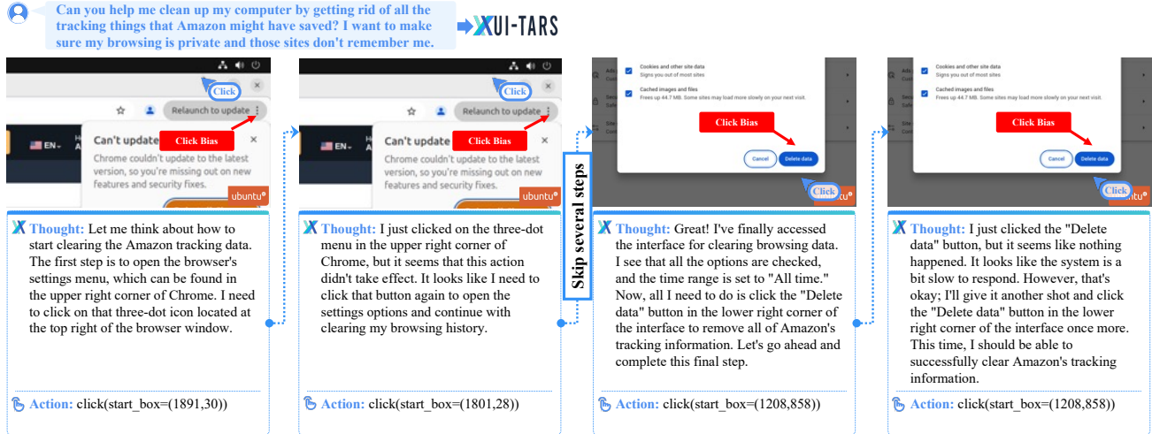
Figure 11. The performance of UI-TARS-1.5-7B when facing resolution change. The click positions deviate from the target positions.
