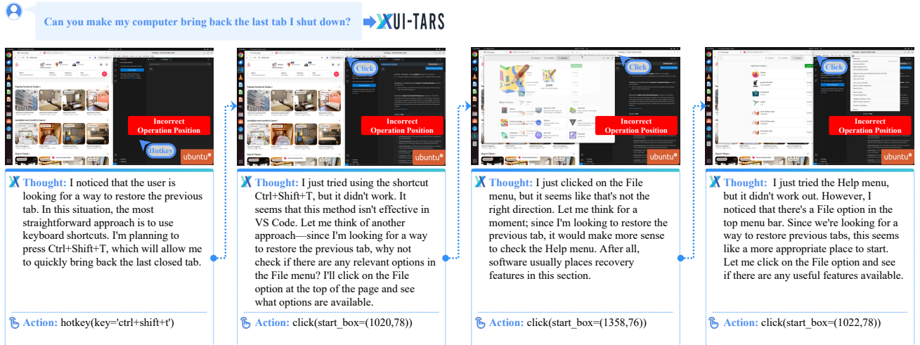
Figure 14. The performance of UI-TARS-1.5-7B when facing multi apps. Agent conduct operations in incorrect positions.
