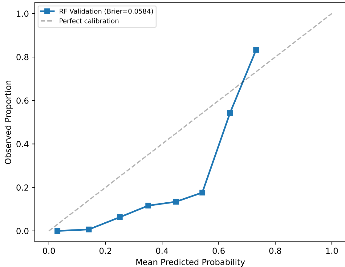
Calibration Plot
